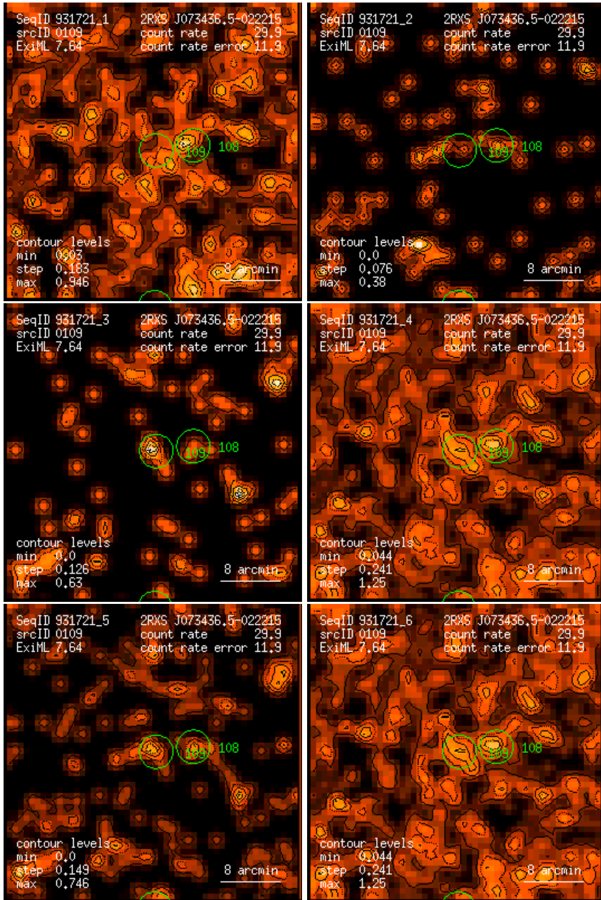
Figure 109: RASS 931721: detection 0109: band rate images, Gaussian filter: (1) PSPC channels 11 – 41, (2) 52 – 90, (3) 91 – 201, (4) 11 – 235, (5) 52 – 201, (6) 11 – 201. Broad band rates in counts/ks. Band rate contour levels in counts/ks/arcmin 2 .
