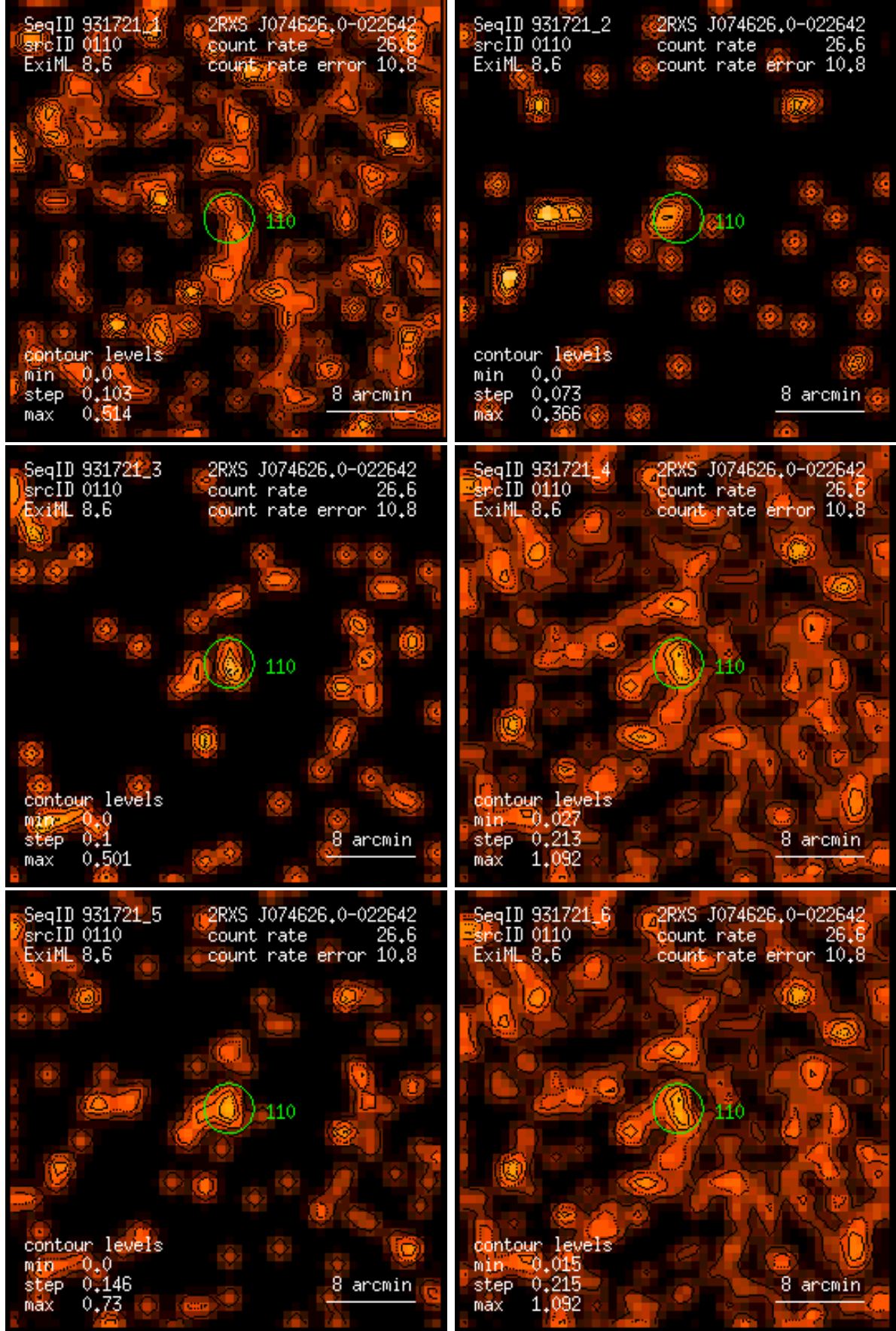
Figure 110: RASS 931721: detection 0110: band rate images, Gaussian filter: (1) PSPC channels 11 – 41, (2) 52 – 90, (3) 91 – 201, (4) 11 – 235, (5) 52 – 201, (6) 11 – 201. Broad band rates in counts/ks. Band rate contour levels in counts/ks/arcmin 2 .
