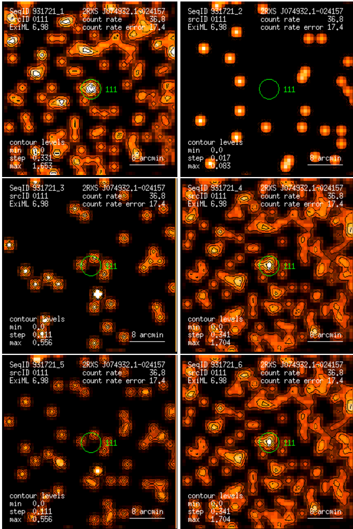
Figure 111: RASS 931721: detection 0111: band rate images, Gaussian filter: (1) PSPC channels 11 – 41, (2) 52 – 90, (3) 91 – 201, (4) 11 – 235, (5) 52 – 201, (6) 11 – 201. Broad band rates in counts/ks. Band rate contour levels in counts/ks/arcmin 2 .
