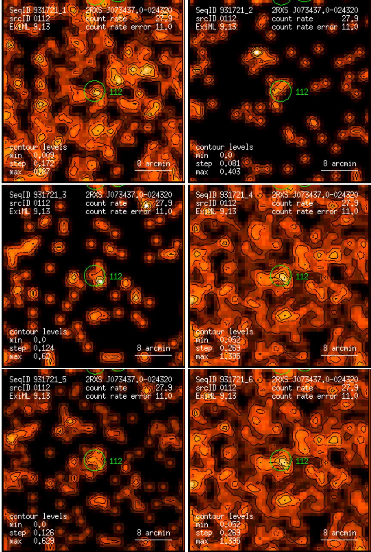
Figure 112: RASS 931721: detection 0112: band rate images, Gaussian filter: (1) PSPC channels 11 – 41, (2) 52 – 90, (3) 91 – 201, (4) 11 – 235, (5) 52 – 201, (6) 11 – 201. Broad band rates in counts/ks. Band rate contour levels in counts/ks/arcmin 2 .
