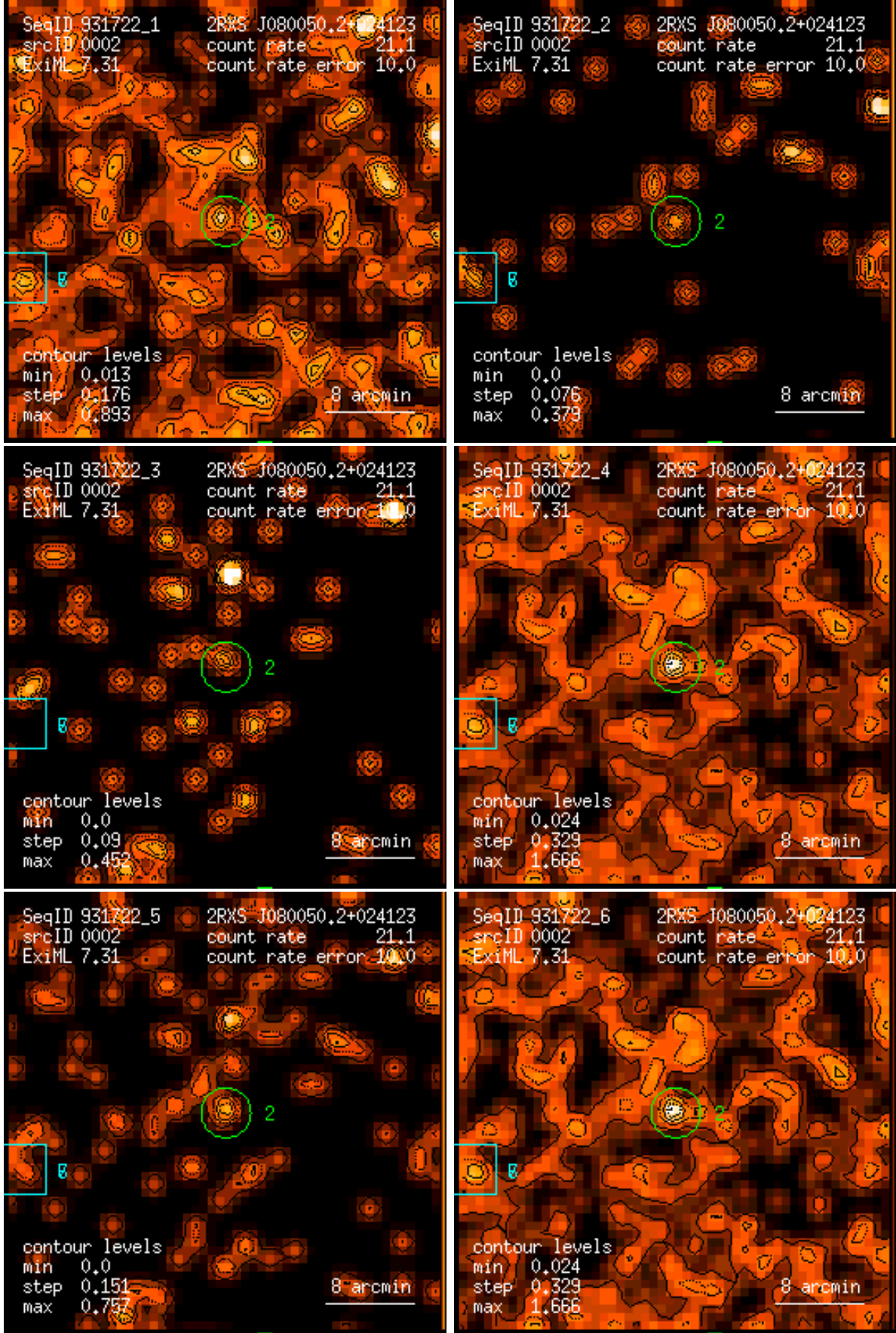
Figure 2: RASS 931722: detection 0002: band rate images, Gaussian filter: (1) PSPC channels 11 – 41, (2) 52 – 90, (3) 91 – 201, (4) 11 – 235, (5) 52 – 201, (6) 11 – 201. Broad band rates in counts/ks. Band rate contour levels in counts/ks/arcmin 2 .
