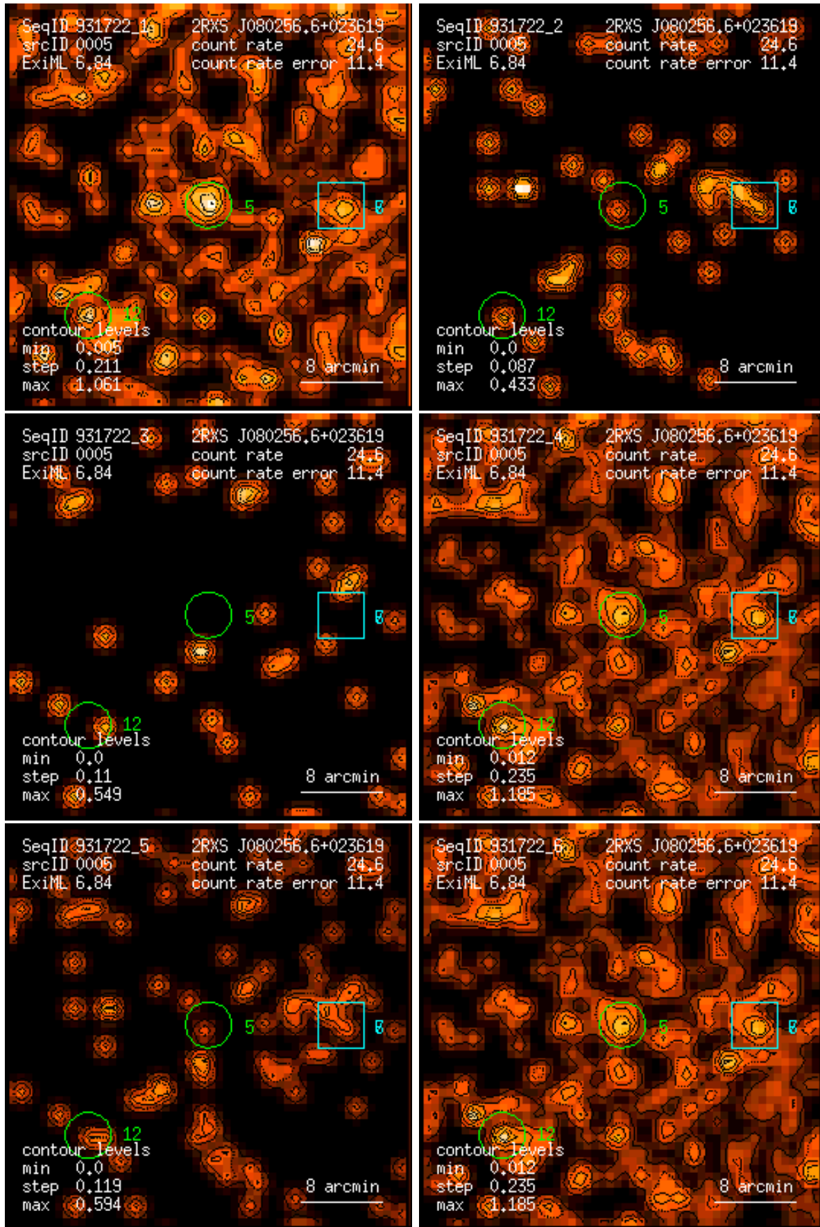
Figure 5: RASS 931722: detection 0005: band rate images, Gaussian filter: (1) PSPC channels 11 – 41, (2) 52 – 90, (3) 91 – 201, (4) 11 – 235, (5) 52 – 201, (6) 11 – 201. Broad band rates in counts/ks. Band rate contour levels in counts/ks/arcmin 2 .
