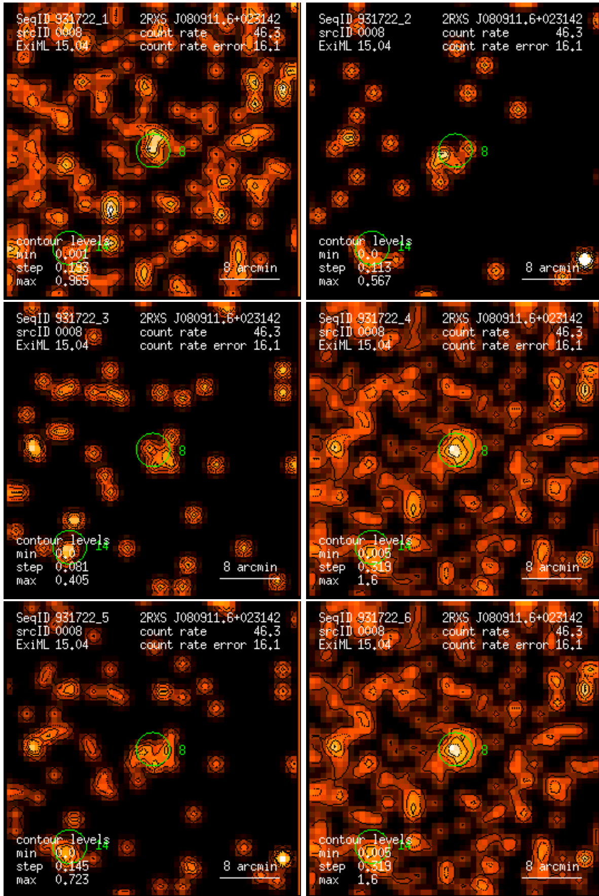
Figure 8: RASS 931722: detection 0008: band rate images, Gaussian filter: (1) PSPC channels 11 – 41, (2) 52 – 90, (3) 91 – 201, (4) 11 – 235, (5) 52 – 201, (6) 11 – 201. Broad band rates in counts/ks. Band rate contour levels in counts/ks/arcmin 2 .
