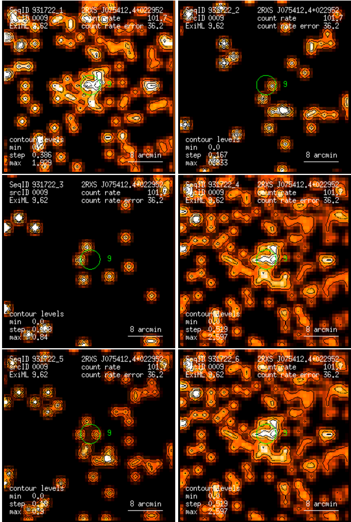
Figure 9: RASS 931722: detection 0009: band rate images, Gaussian filter: (1) PSPC channels 11 – 41, (2) 52 – 90, (3) 91 – 201, (4) 11 – 235, (5) 52 – 201, (6) 11 – 201. Broad band rates in counts/ks. Band rate contour levels in counts/ks/arcmin 2 .
