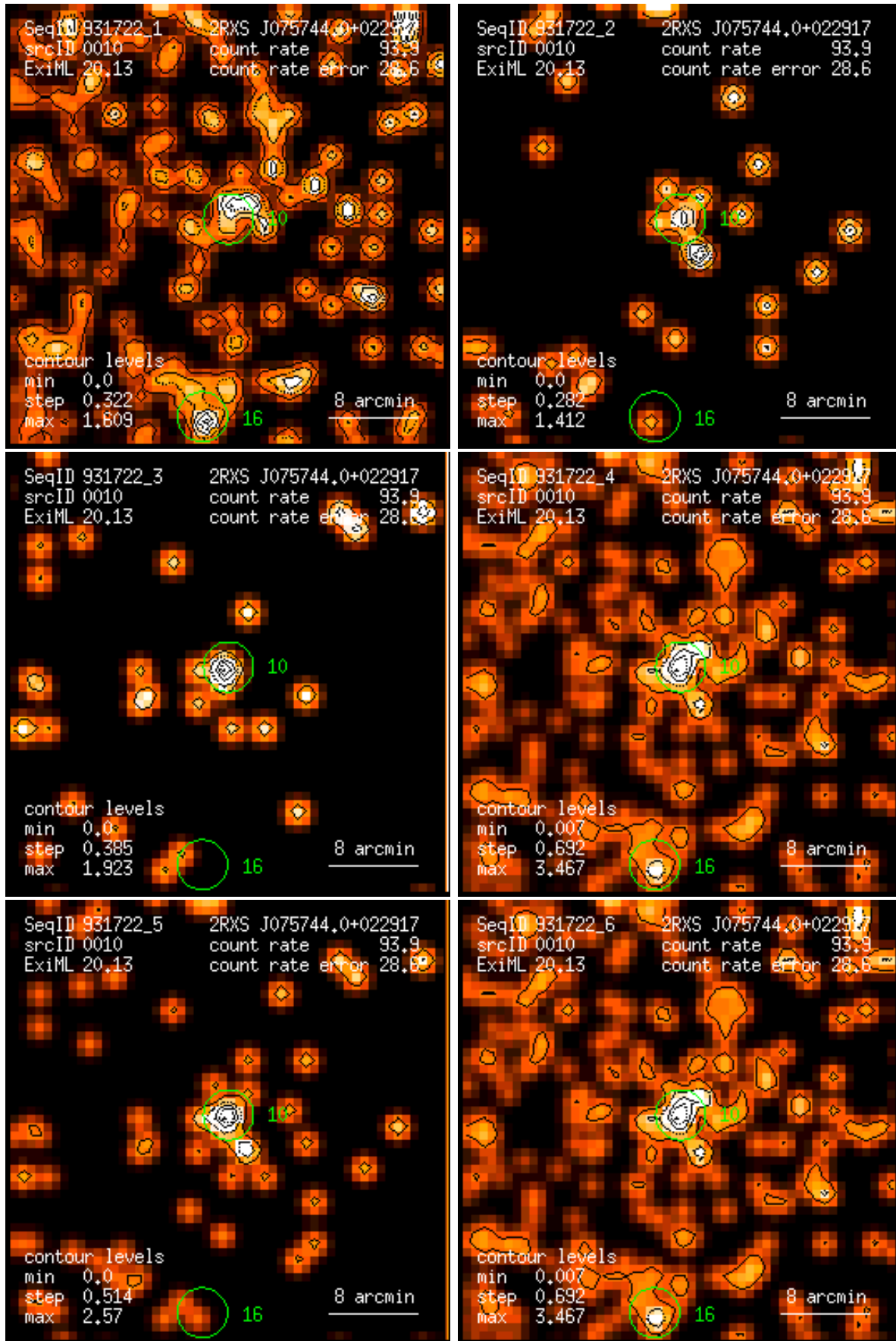
Figure 10: RASS 931722: detection 0010: band rate images, Gaussian filter: (1) PSPC channels 11 – 41, (2) 52 – 90, (3) 91 – 201, (4) 11 – 235, (5) 52 – 201, (6) 11 – 201. Broad band rates in counts/ks. Band rate contour levels in counts/ks/arcmin 2 .
