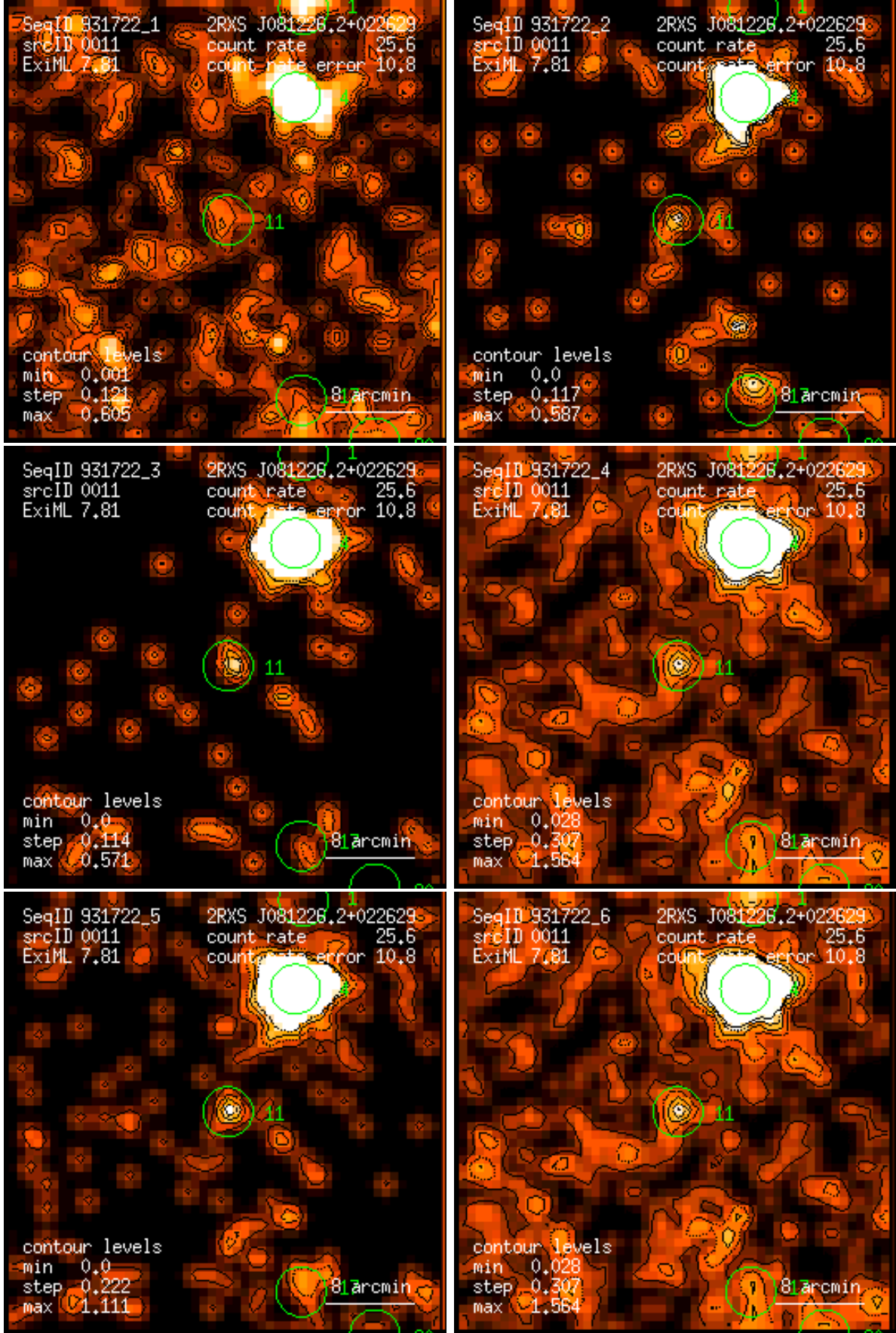
Figure 11: RASS 931722: detection 0011: band rate images, Gaussian filter: (1) PSPC channels 11 – 41, (2) 52 – 90, (3) 91 – 201, (4) 11 – 235, (5) 52 – 201, (6) 11 – 201. Broad band rates in counts/ks. Band rate contour levels in counts/ks/arcmin 2 .
