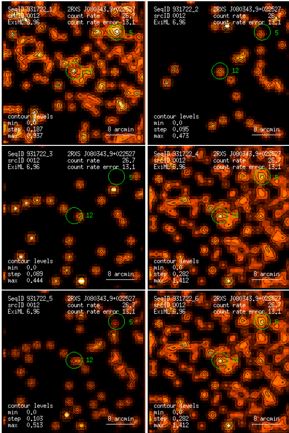
Figure 12: RASS 931722: detection 0012: band rate images, Gaussian filter: (1) PSPC channels 11 – 41, (2) 52 – 90, (3) 91 – 201, (4) 11 – 235, (5) 52 – 201, (6) 11 – 201. Broad band rates in counts/ks. Band rate contour levels in counts/ks/arcmin 2 .
