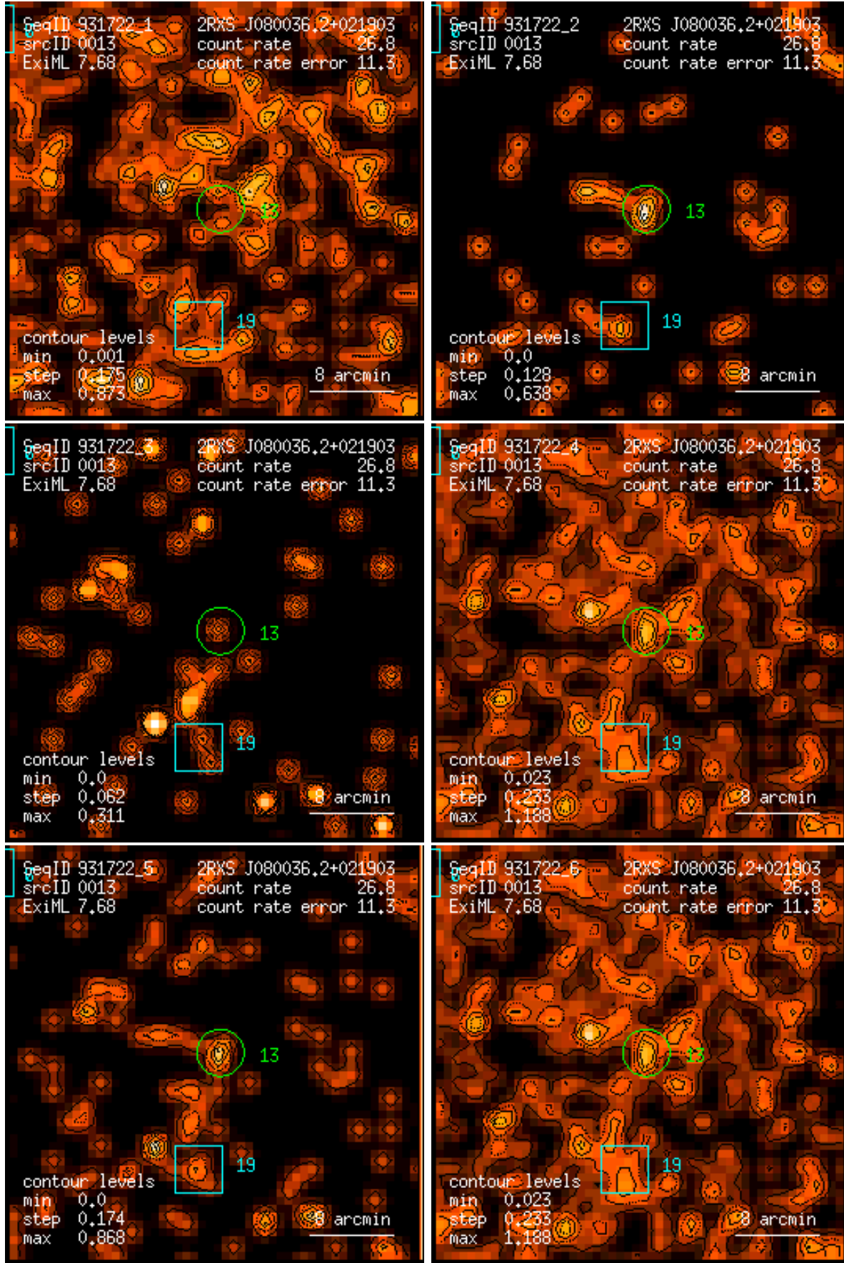
Figure 13: RASS 931722: detection 0013: band rate images, Gaussian filter: (1) PSPC channels 11 – 41, (2) 52 – 90, (3) 91 – 201, (4) 11 – 235, (5) 52 – 201, (6) 11 – 201. Broad band rates in counts/ks. Band rate contour levels in counts/ks/arcmin 2 .
