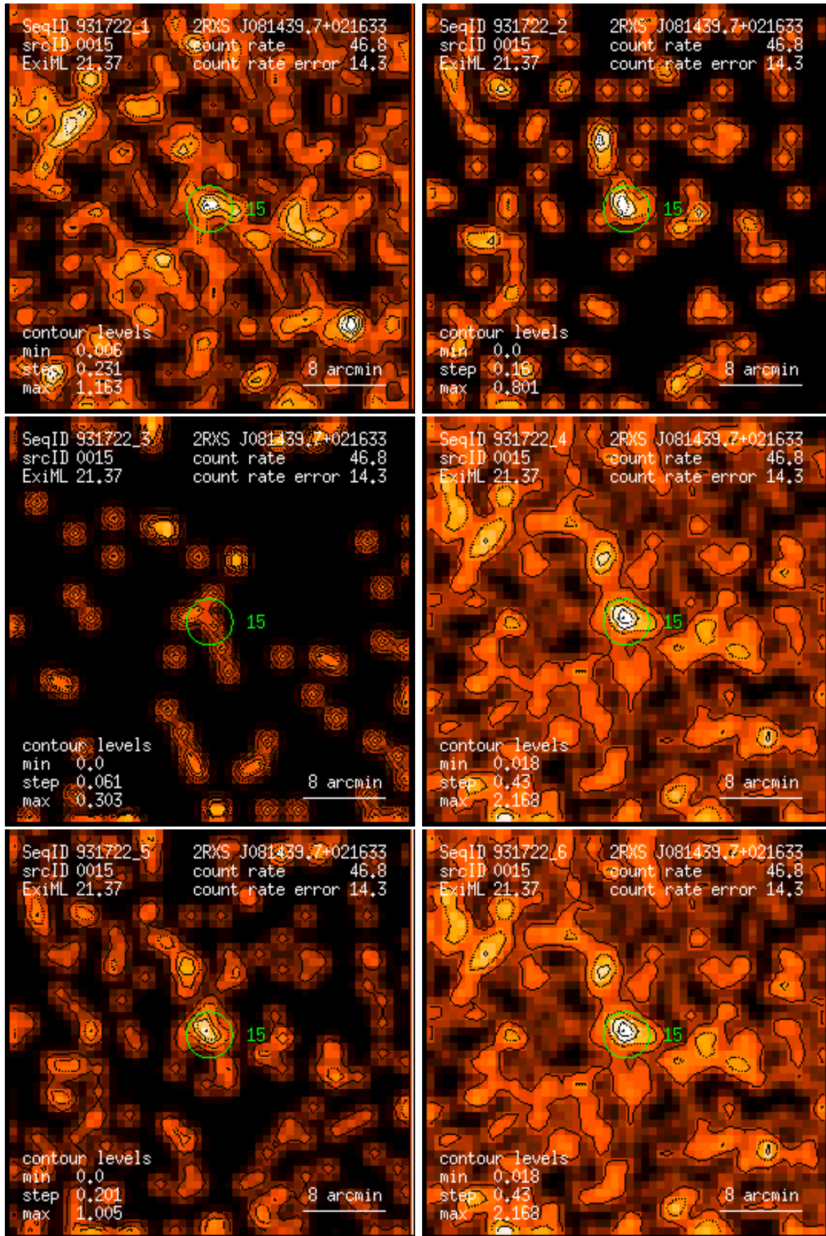
Figure 15: RASS 931722: detection 0015: band rate images, Gaussian filter: (1) PSPC channels 11 – 41, (2) 52 – 90, (3) 91 – 201, (4) 11 – 235, (5) 52 – 201, (6) 11 – 201. Broad band rates in counts/ks. Band rate contour levels in counts/ks/arcmin 2 .
