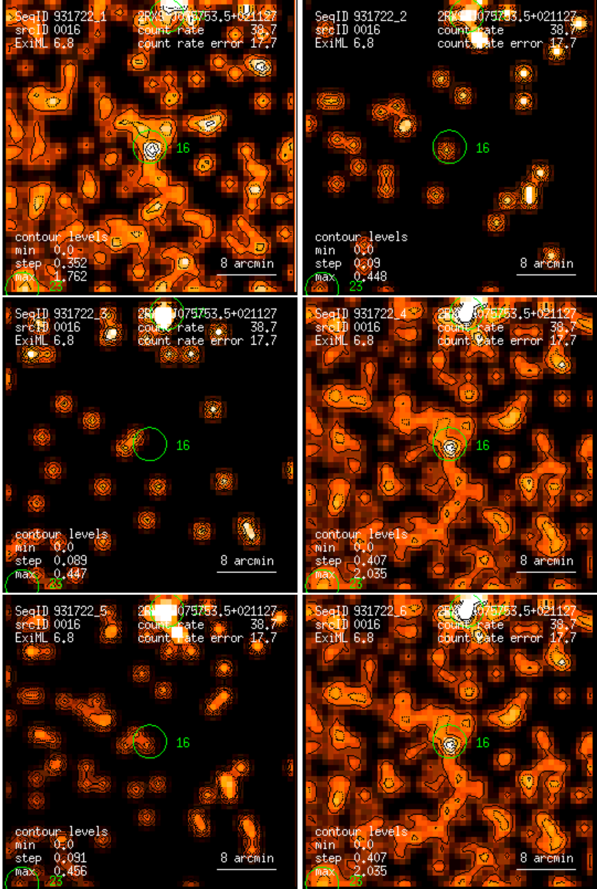
Figure 16: RASS 931722: detection 0016: band rate images, Gaussian filter: (1) PSPC channels 11 – 41, (2) 52 – 90, (3) 91 – 201, (4) 11 – 235, (5) 52 – 201, (6) 11 – 201. Broad band rates in counts/ks. Band rate contour levels in counts/ks/arcmin 2 .
