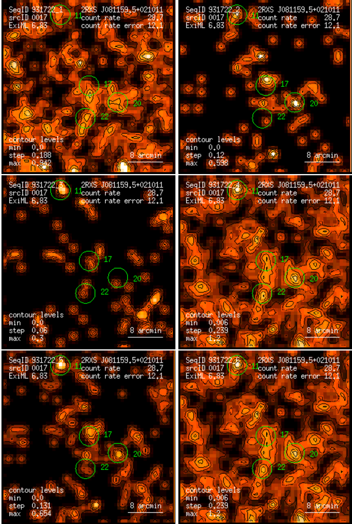
Figure 17: RASS 931722: detection 0017: band rate images, Gaussian filter: (1) PSPC channels 11 – 41, (2) 52 – 90, (3) 91 – 201, (4) 11 – 235, (5) 52 – 201, (6) 11 – 201. Broad band rates in counts/ks. Band rate contour levels in counts/ks/arcmin 2 .
