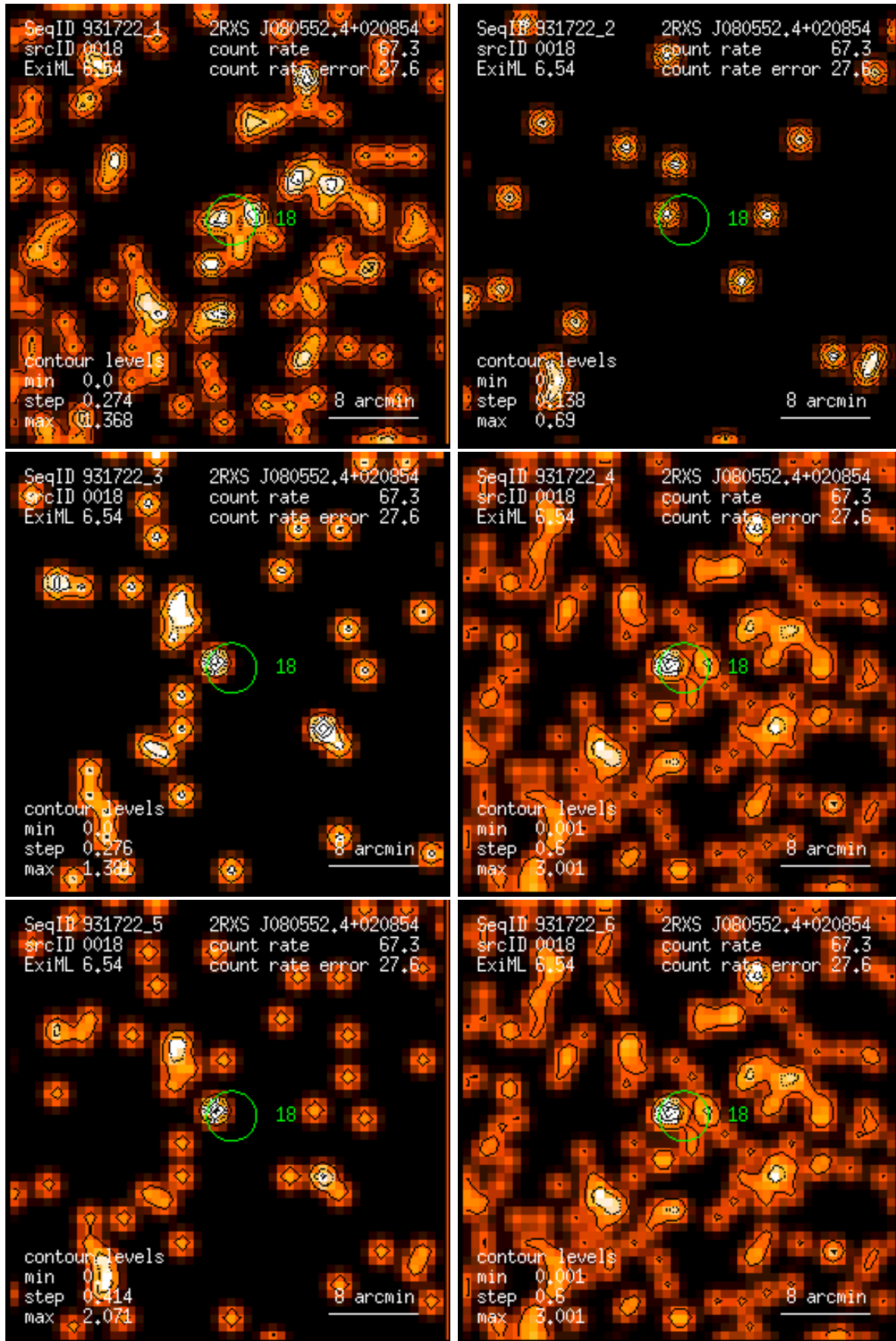
Figure 18: RASS 931722: detection 0018: band rate images, Gaussian filter: (1) PSPC channels 11 – 41, (2) 52 – 90, (3) 91 – 201, (4) 11 – 235, (5) 52 – 201, (6) 11 – 201. Broad band rates in counts/ks. Band rate contour levels in counts/ks/arcmin 2 .
