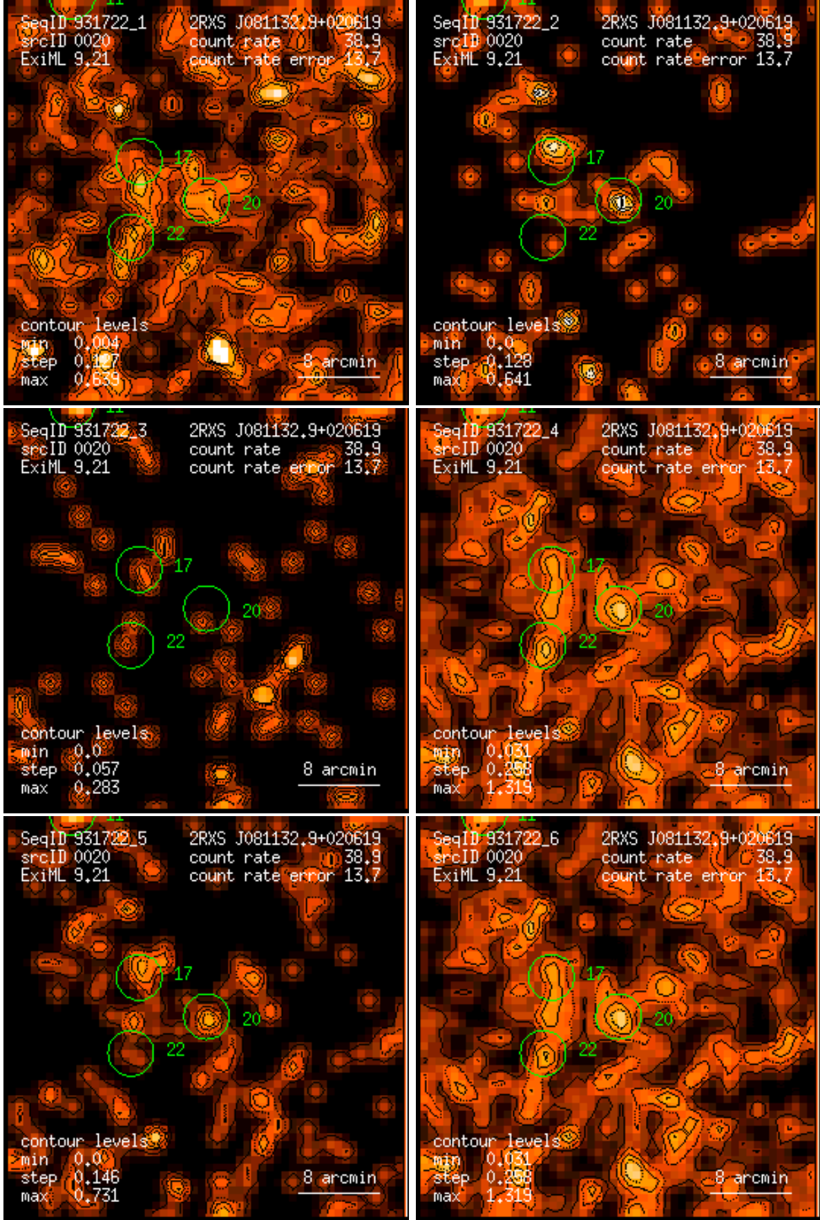
Figure 20: RASS 931722: detection 0020: band rate images, Gaussian filter: (1) PSPC channels 11 – 41, (2) 52 – 90, (3) 91 – 201, (4) 11 – 235, (5) 52 – 201, (6) 11 – 201. Broad band rates in counts/ks. Band rate contour levels in counts/ks/arcmin 2 .
