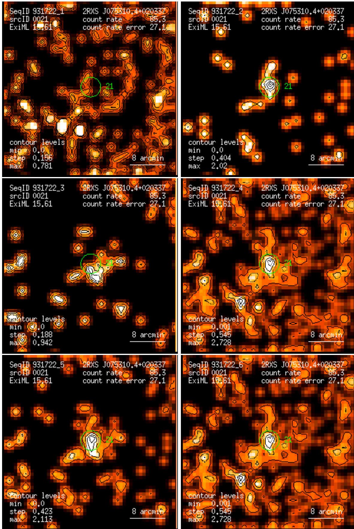
Figure 21: RASS 931722: detection 0021: band rate images, Gaussian filter: (1) PSPC channels 11 – 41, (2) 52 – 90, (3) 91 – 201, (4) 11 – 235, (5) 52 – 201, (6) 11 – 201. Broad band rates in counts/ks. Band rate contour levels in counts/ks/arcmin 2 .
