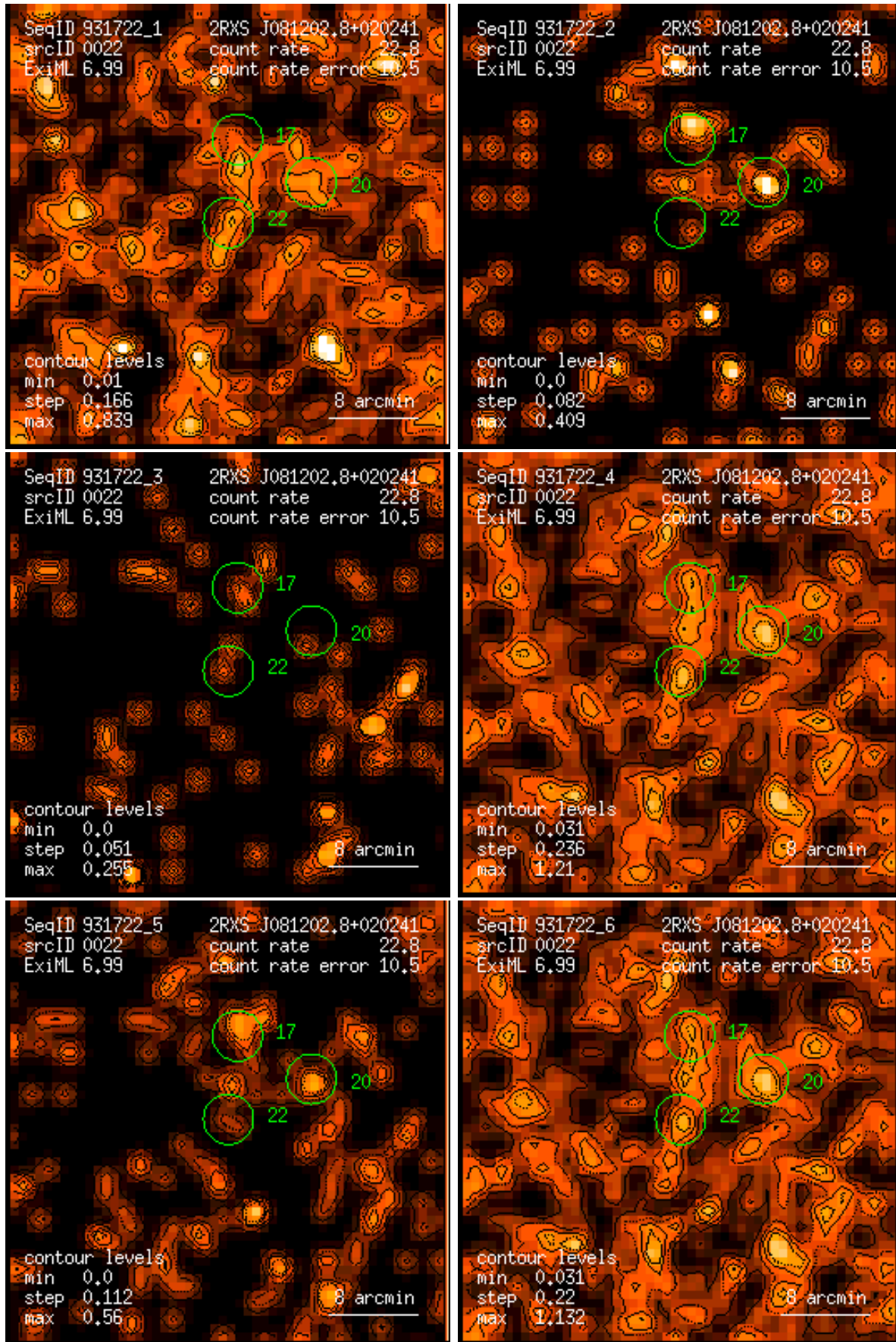
Figure 22: RASS 931722: detection 0022: band rate images, Gaussian filter: (1) PSPC channels 11 – 41, (2) 52 – 90, (3) 91 – 201, (4) 11 – 235, (5) 52 – 201, (6) 11 – 201. Broad band rates in counts/ks. Band rate contour levels in counts/ks/arcmin 2 .
