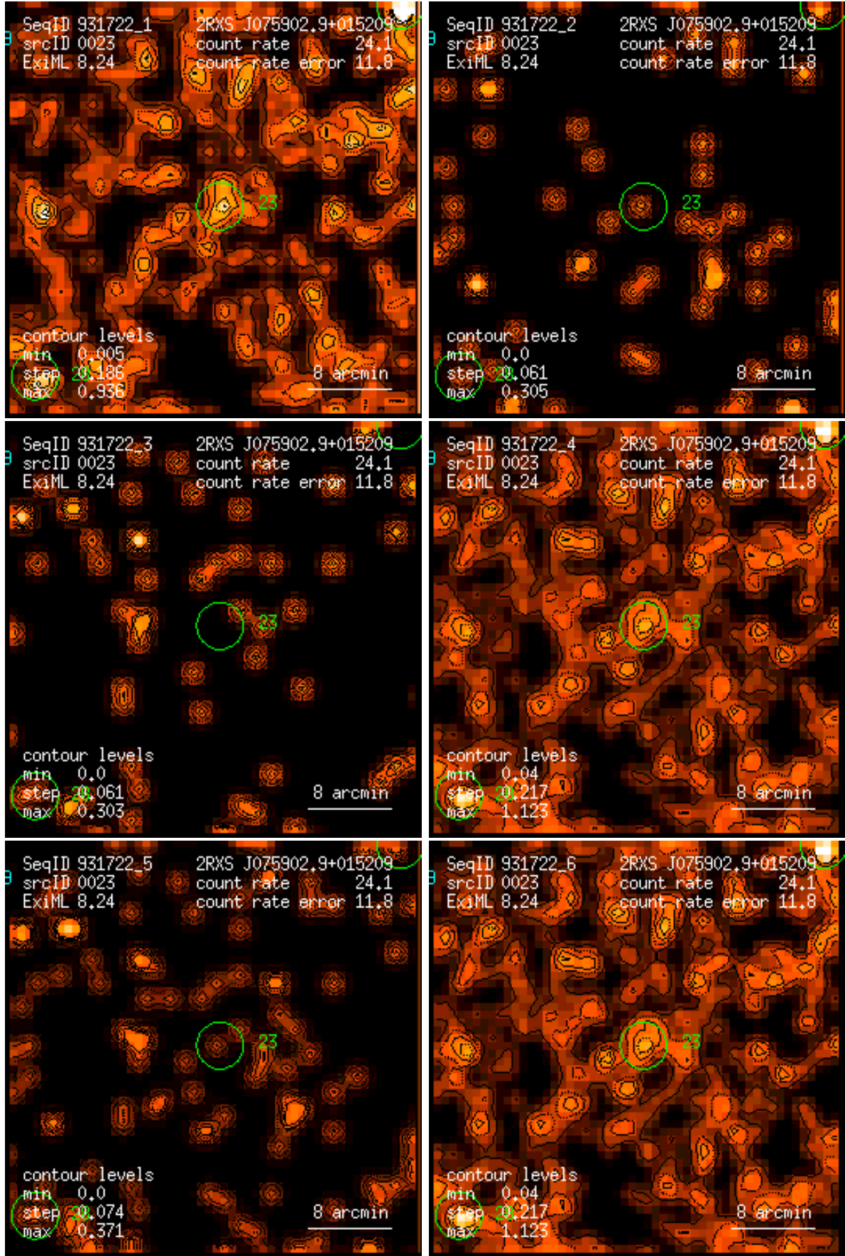
Figure 23: RASS 931722: detection 0023: band rate images, Gaussian filter: (1) PSPC channels 11 – 41, (2) 52 – 90, (3) 91 – 201, (4) 11 – 235, (5) 52 – 201, (6) 11 – 201. Broad band rates in counts/ks. Band rate contour levels in counts/ks/arcmin 2 .
