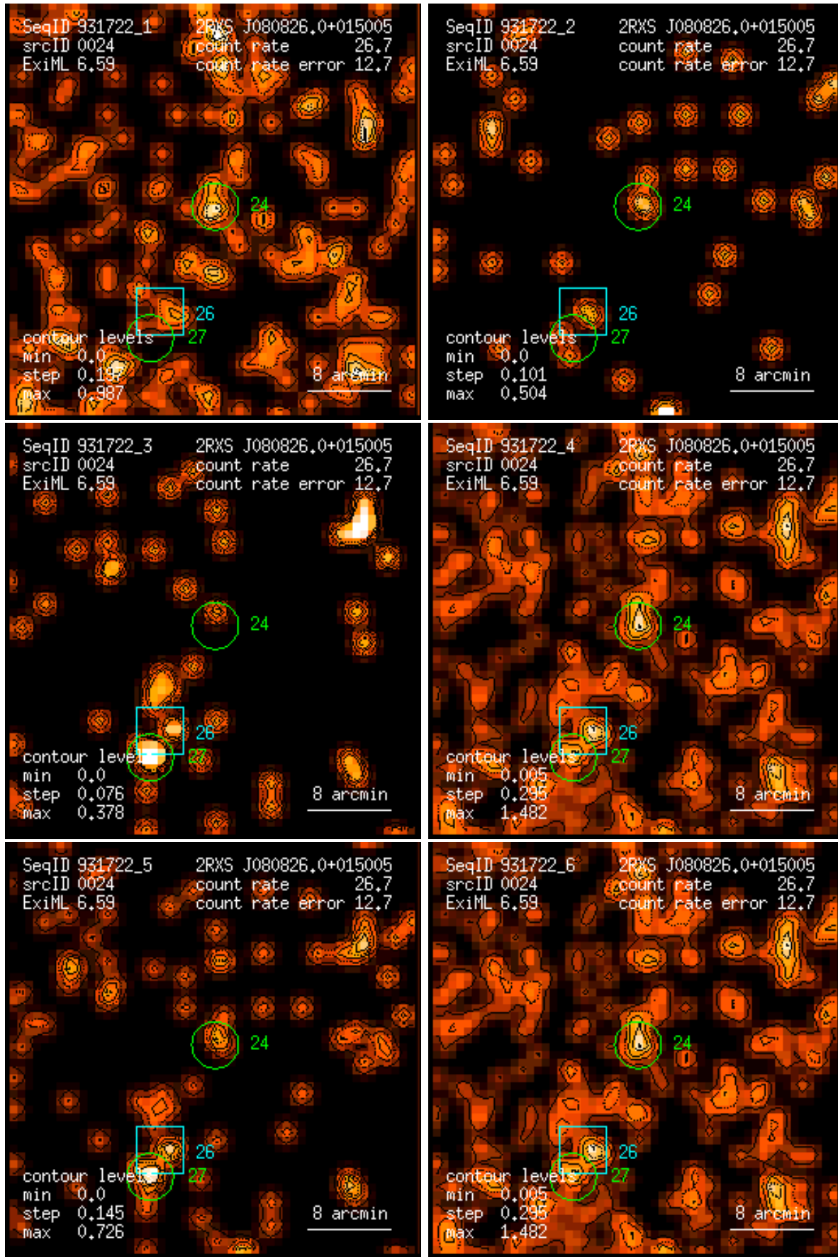
Figure 24: RASS 931722: detection 0024: band rate images, Gaussian filter: (1) PSPC channels 11 – 41, (2) 52 – 90, (3) 91 – 201, (4) 11 – 235, (5) 52 – 201, (6) 11 – 201. Broad band rates in counts/ks. Band rate contour levels in counts/ks/arcmin 2 .
