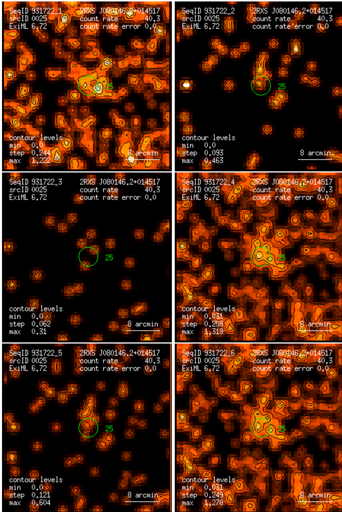
Figure 25: RASS 931722: detection 0025: band rate images, Gaussian filter: (1) PSPC channels 11 – 41, (2) 52 – 90, (3) 91 – 201, (4) 11 – 235, (5) 52 – 201, (6) 11 – 201. Broad band rates in counts/ks. Band rate contour levels in counts/ks/arcmin 2 .
