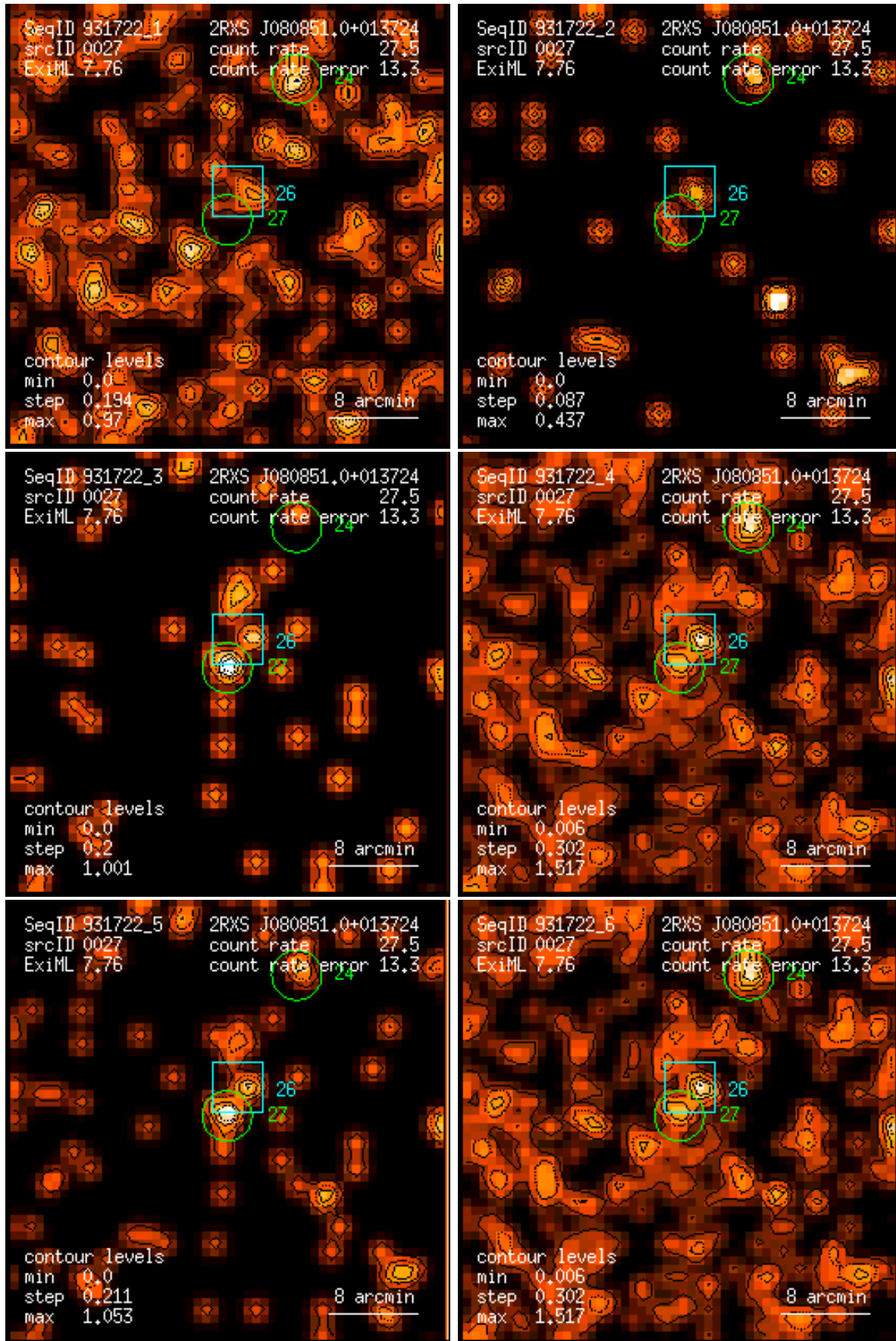
Figure 27: RASS 931722: detection 0027: band rate images, Gaussian filter: (1) PSPC channels 11 – 41, (2) 52 – 90, (3) 91 – 201, (4) 11 – 235, (5) 52 – 201, (6) 11 – 201. Broad band rates in counts/ks. Band rate contour levels in counts/ks/arcmin 2 .
