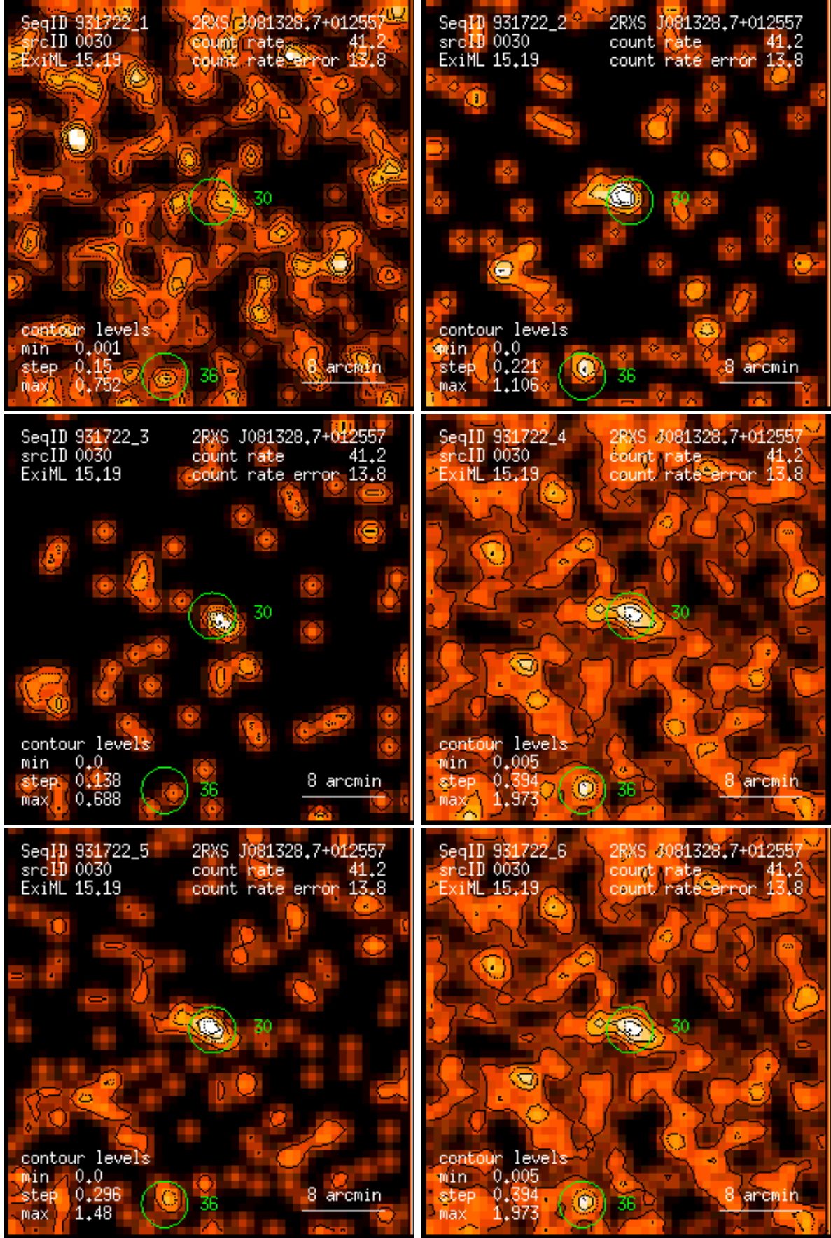
Figure 30: RASS 931722: detection 0030: band rate images, Gaussian filter: (1) PSPC channels 11 – 41, (2) 52 – 90, (3) 91 – 201, (4) 11 – 235, (5) 52 – 201, (6) 11 – 201. Broad band rates in counts/ks. Band rate contour levels in counts/ks/arcmin 2 .
