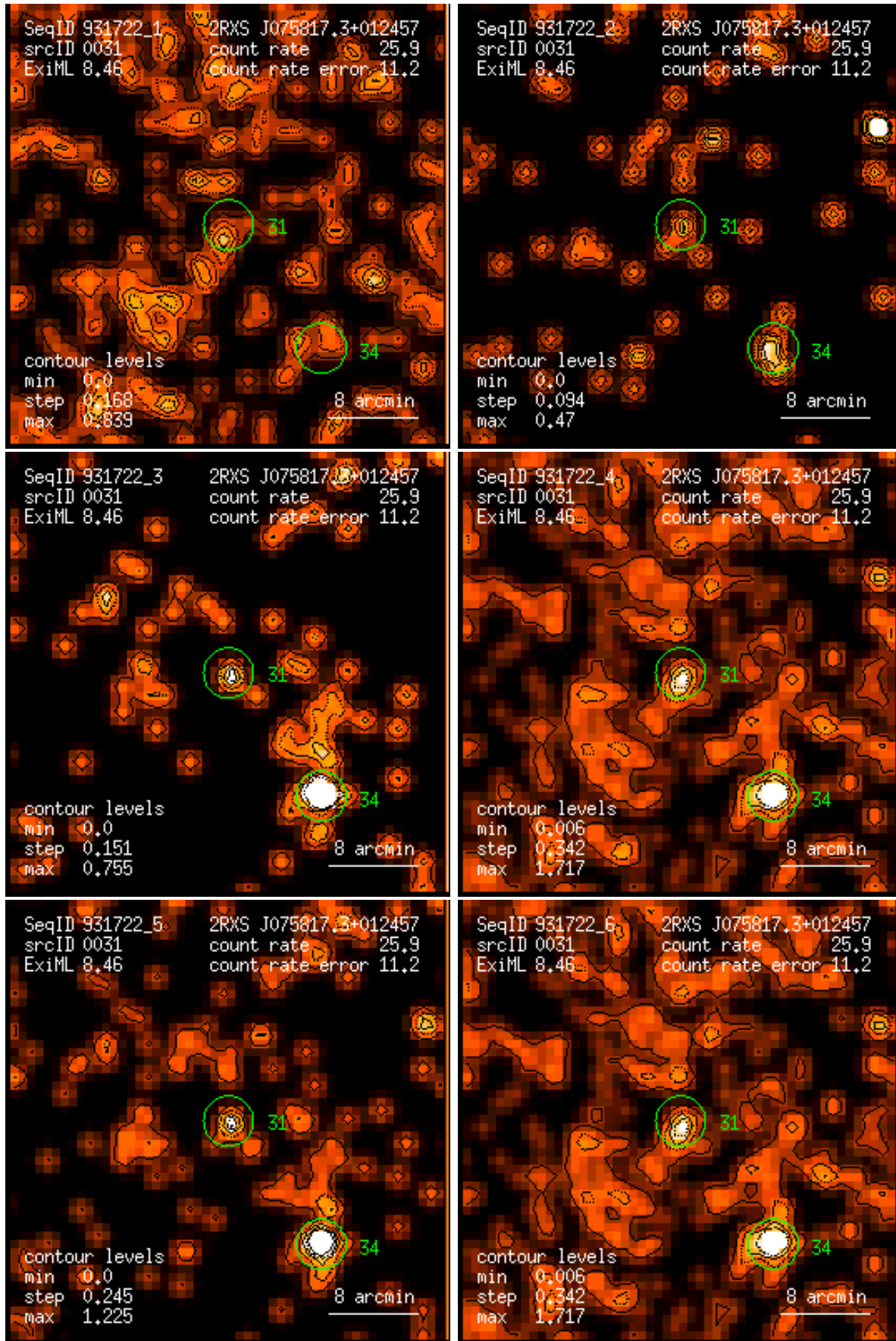
Figure 31: RASS 931722: detection 0031: band rate images, Gaussian filter: (1) PSPC channels 11 – 41, (2) 52 – 90, (3) 91 – 201, (4) 11 – 235, (5) 52 – 201, (6) 11 – 201. Broad band rates in counts/ks. Band rate contour levels in counts/ks/arcmin 2 .
