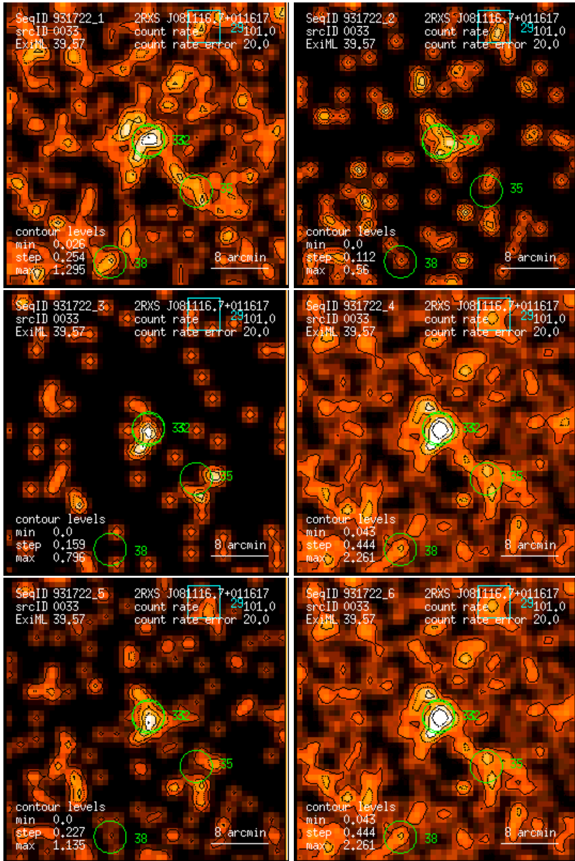
Figure 33: RASS 931722: detection 0033: band rate images, Gaussian filter: (1) PSPC channels 11 – 41, (2) 52 – 90, (3) 91 – 201, (4) 11 – 235, (5) 52 – 201, (6) 11 – 201. Broad band rates in counts/ks. Band rate contour levels in counts/ks/arcmin 2 .
