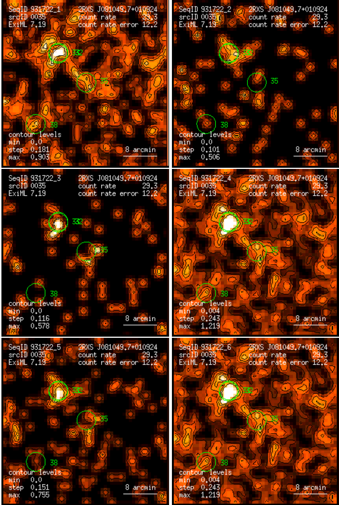
Figure 35: RASS 931722: detection 0035: band rate images, Gaussian filter: (1) PSPC channels 11 – 41, (2) 52 – 90, (3) 91 – 201, (4) 11 – 235, (5) 52 – 201, (6) 11 – 201. Broad band rates in counts/ks. Band rate contour levels in counts/ks/arcmin 2 .
