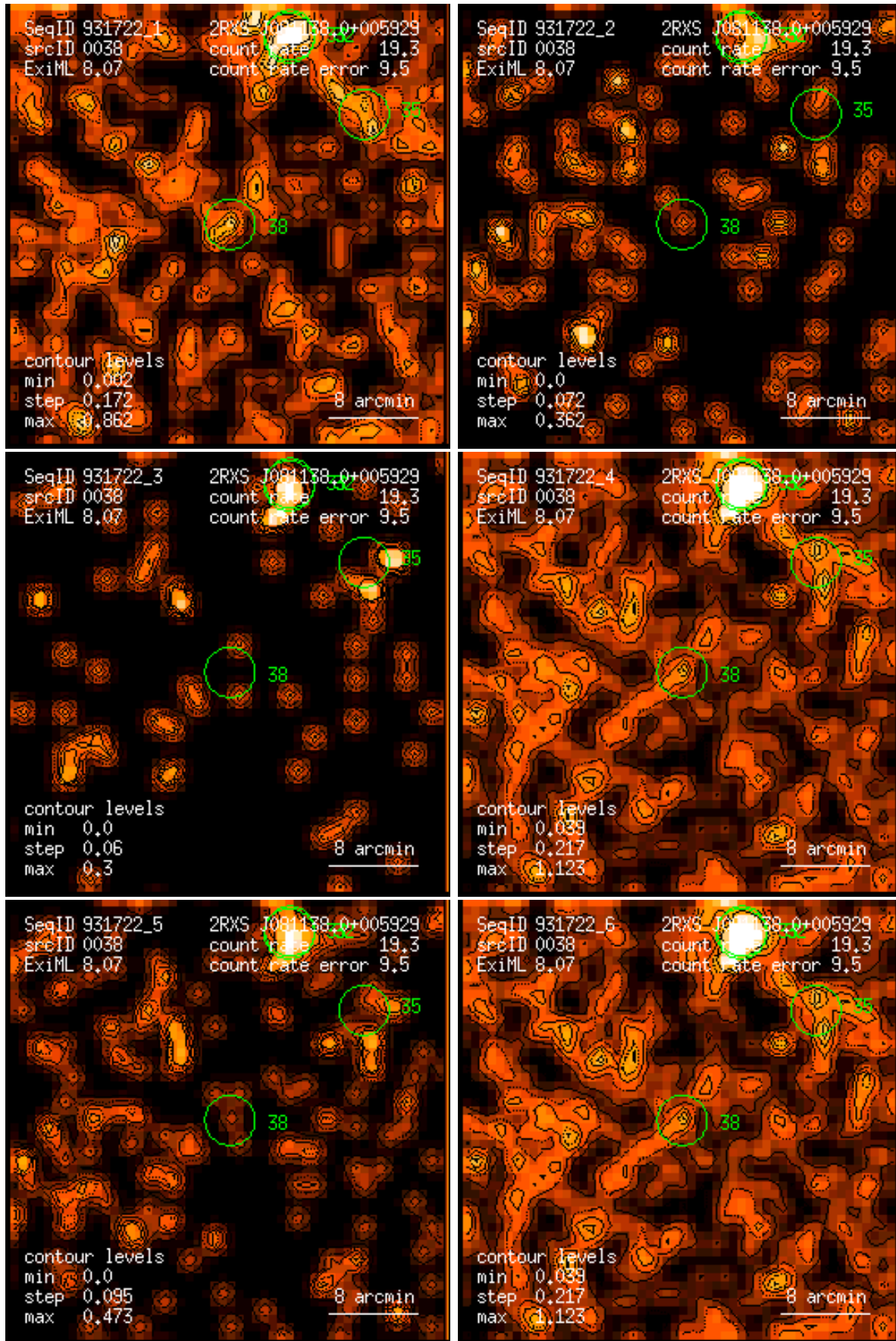
Figure 38: RASS 931722: detection 0038: band rate images, Gaussian filter: (1) PSPC channels 11 – 41, (2) 52 – 90, (3) 91 – 201, (4) 11 – 235, (5) 52 – 201, (6) 11 – 201. Broad band rates in counts/ks. Band rate contour levels in counts/ks/arcmin 2 .
