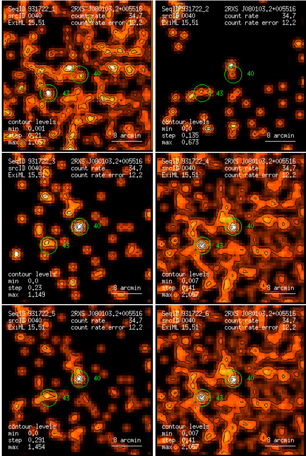
Figure 40: RASS 931722: detection 0040: band rate images, Gaussian filter: (1) PSPC channels 11 – 41, (2) 52 – 90, (3) 91 – 201, (4) 11 – 235, (5) 52 – 201, (6) 11 – 201. Broad band rates in counts/ks. Band rate contour levels in counts/ks/arcmin 2 .
