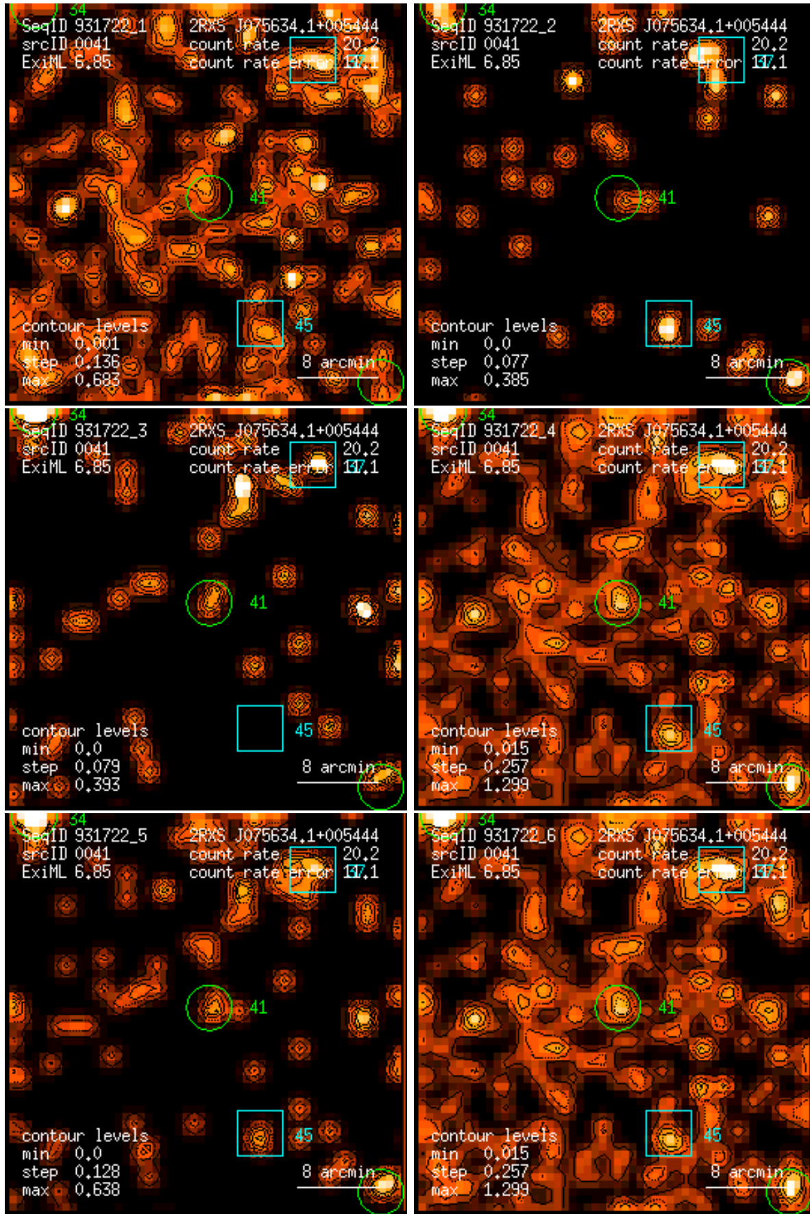
Figure 41: RASS 931722: detection 0041: band rate images, Gaussian filter: (1) PSPC channels 11 – 41, (2) 52 – 90, (3) 91 – 201, (4) 11 – 235, (5) 52 – 201, (6) 11 – 201. Broad band rates in counts/ks. Band rate contour levels in counts/ks/arcmin 2 .
