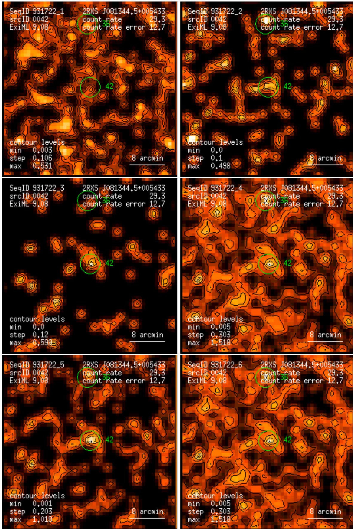
Figure 42: RASS 931722: detection 0042: band rate images, Gaussian filter: (1) PSPC channels 11 – 41, (2) 52 – 90, (3) 91 – 201, (4) 11 – 235, (5) 52 – 201, (6) 11 – 201. Broad band rates in counts/ks. Band rate contour levels in counts/ks/arcmin 2 .
