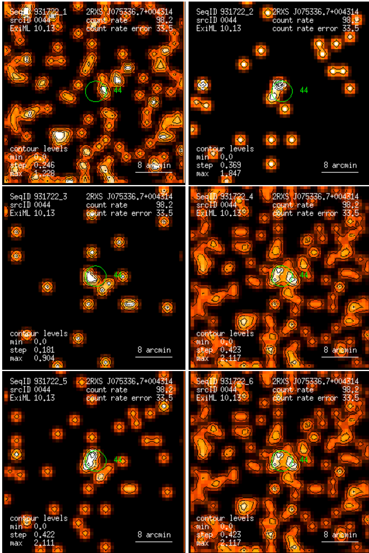
Figure 44: RASS 931722: detection 0044: band rate images, Gaussian filter: (1) PSPC channels 11 – 41, (2) 52 – 90, (3) 91 – 201, (4) 11 – 235, (5) 52 – 201, (6) 11 – 201. Broad band rates in counts/ks. Band rate contour levels in counts/ks/arcmin 2 .
