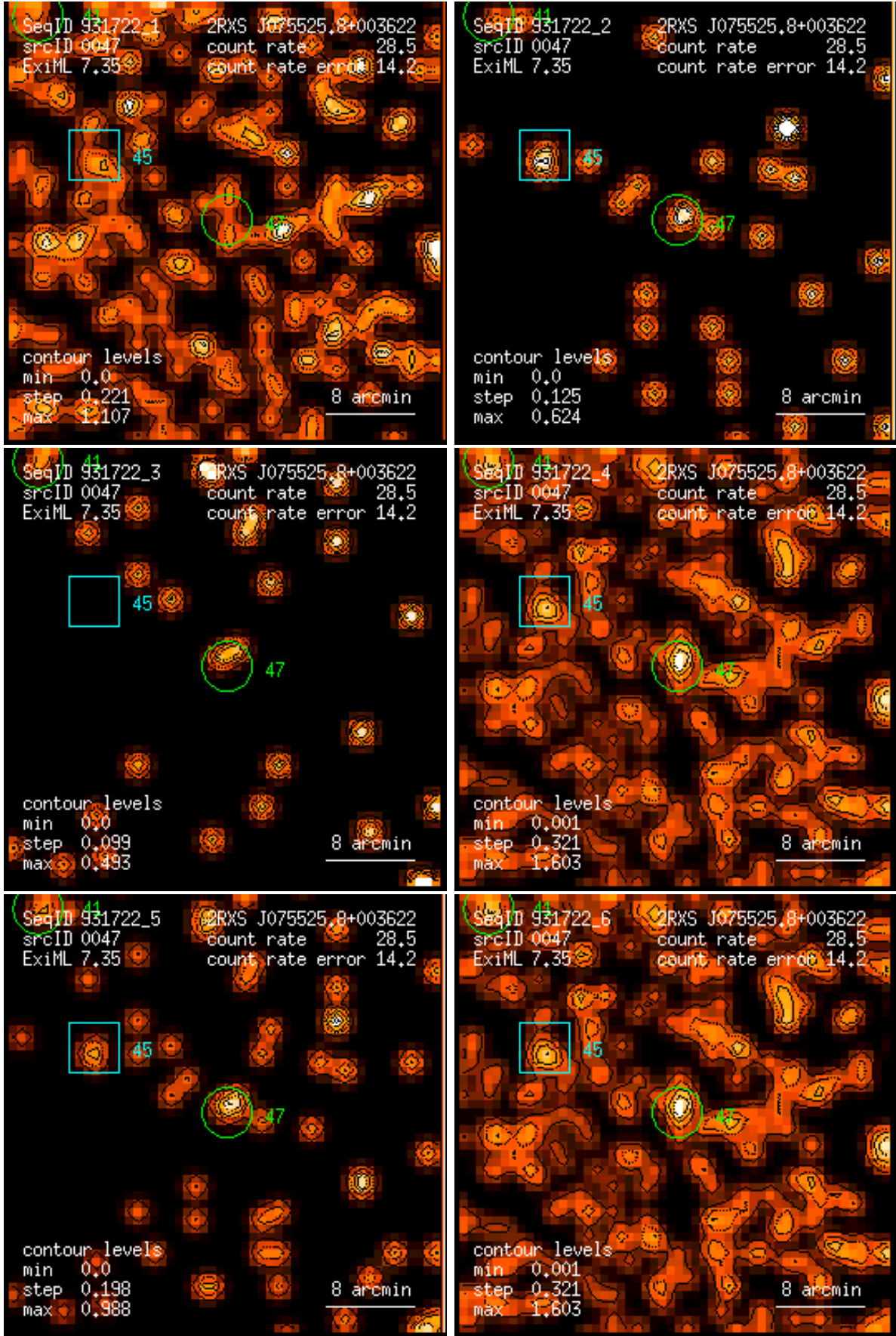
Figure 47: RASS 931722: detection 0047: band rate images, Gaussian filter: (1) PSPC channels 11 – 41, (2) 52 – 90, (3) 91 – 201, (4) 11 – 235, (5) 52 – 201, (6) 11 – 201. Broad band rates in counts/ks. Band rate contour levels in counts/ks/arcmin 2 .
