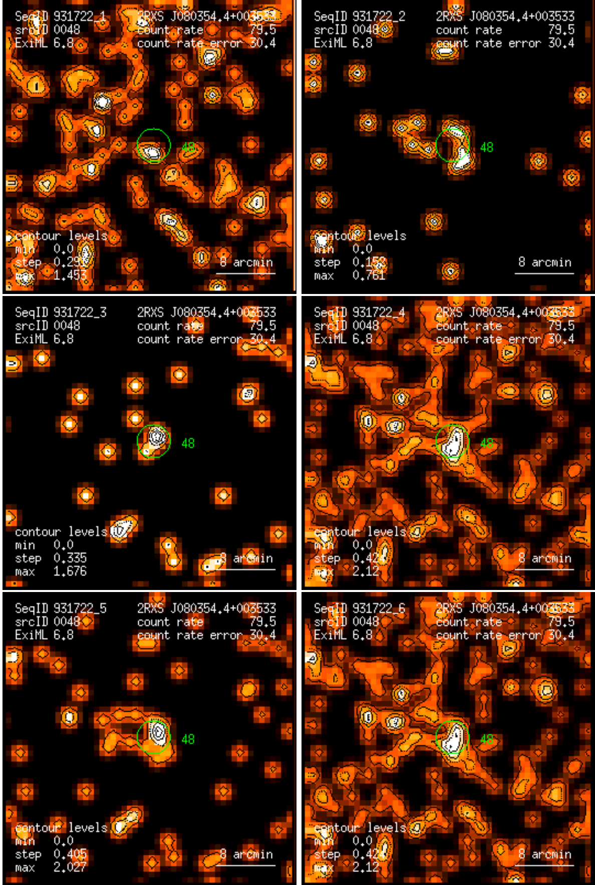
Figure 48: RASS 931722: detection 0048: band rate images, Gaussian filter: (1) PSPC channels 11 – 41, (2) 52 – 90, (3) 91 – 201, (4) 11 – 235, (5) 52 – 201, (6) 11 – 201. Broad band rates in counts/ks. Band rate contour levels in counts/ks/arcmin 2 .
