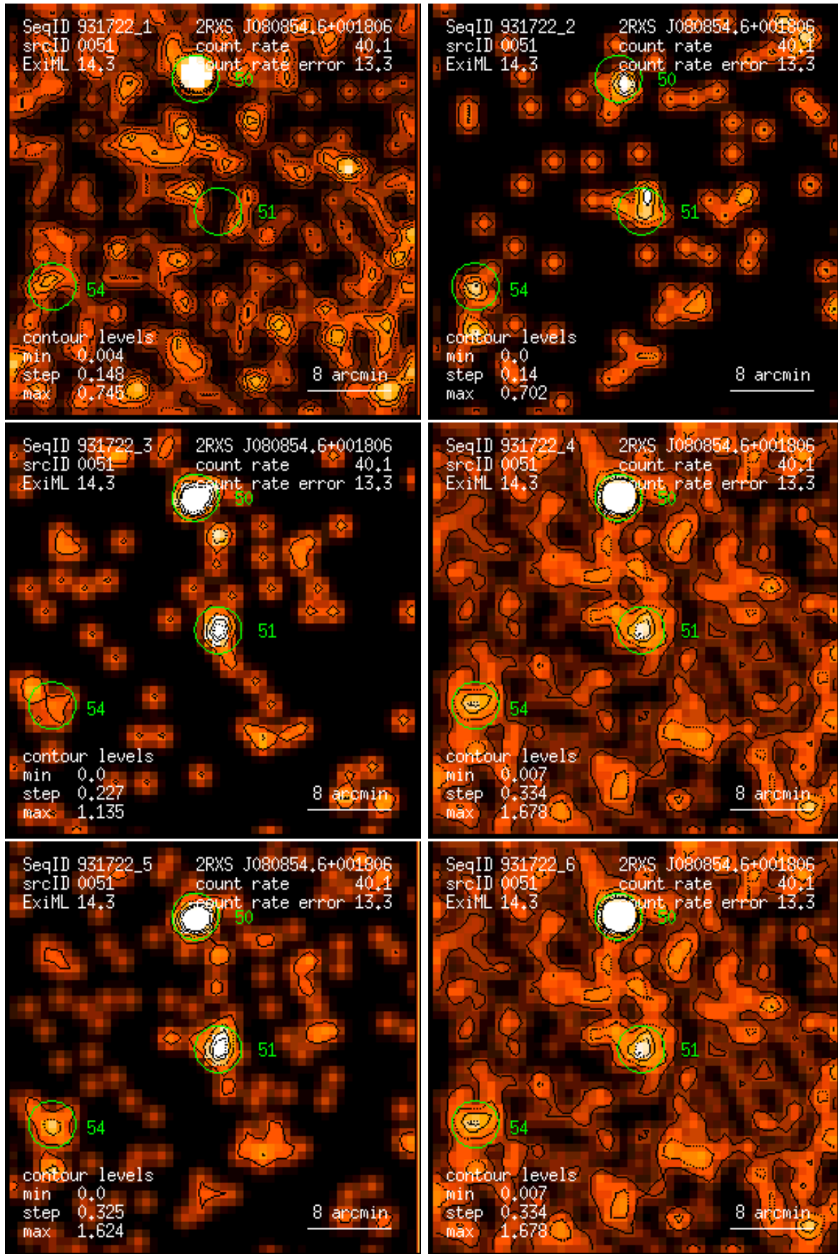
Figure 51: RASS 931722: detection 0051: band rate images, Gaussian filter: (1) PSPC channels 11 – 41, (2) 52 – 90, (3) 91 – 201, (4) 11 – 235, (5) 52 – 201, (6) 11 – 201. Broad band rates in counts/ks. Band rate contour levels in counts/ks/arcmin 2 .
