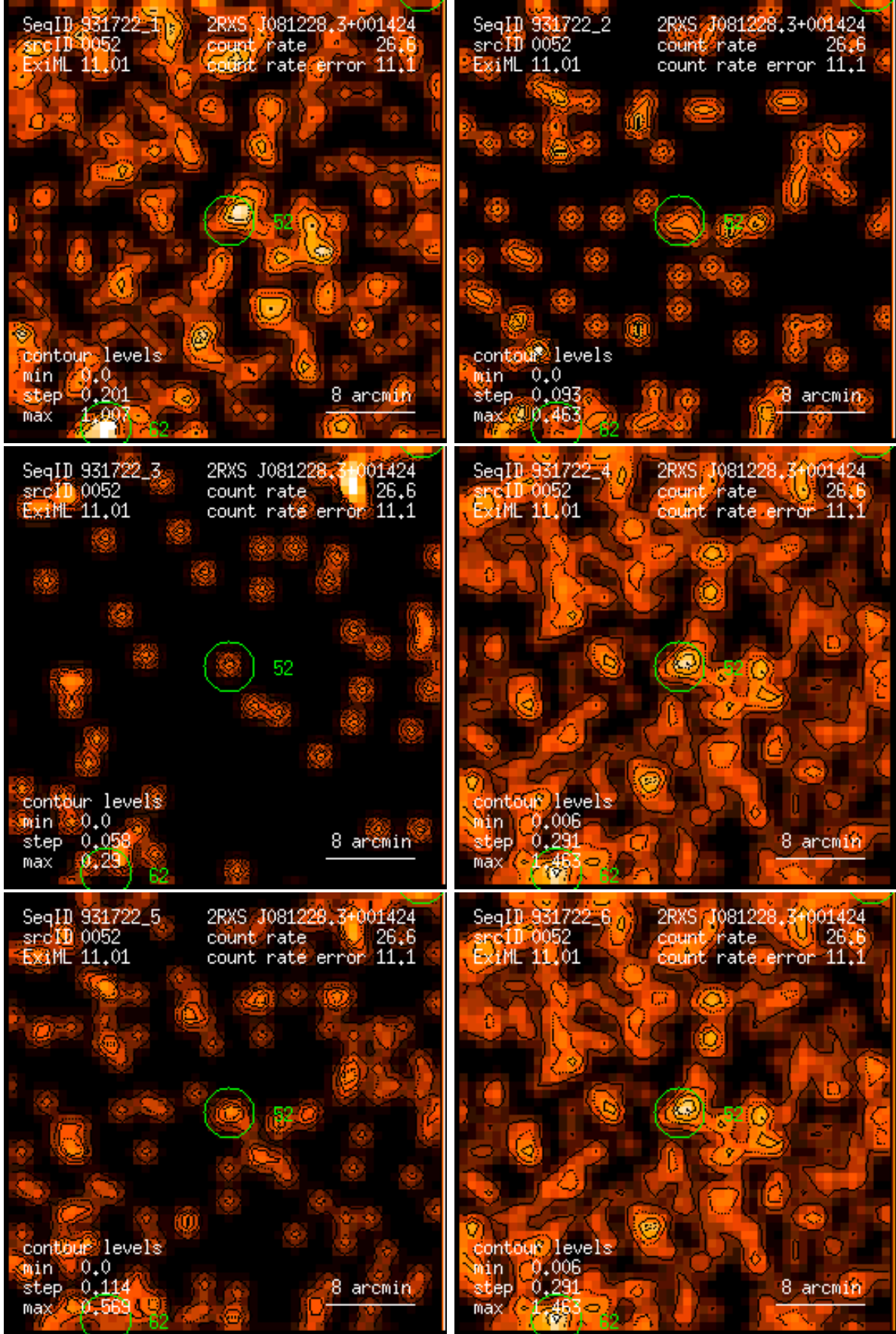
Figure 52: RASS 931722: detection 0052: band rate images, Gaussian filter: (1) PSPC channels 11 – 41, (2) 52 – 90, (3) 91 – 201, (4) 11 – 235, (5) 52 – 201, (6) 11 – 201. Broad band rates in counts/ks. Band rate contour levels in counts/ks/arcmin 2 .
