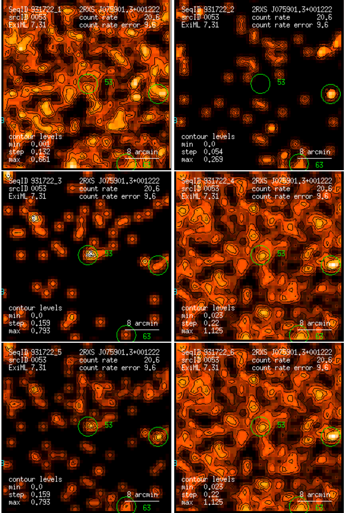
Figure 53: RASS 931722: detection 0053: band rate images, Gaussian filter: (1) PSPC channels 11 – 41, (2) 52 – 90, (3) 91 – 201, (4) 11 – 235, (5) 52 – 201, (6) 11 – 201. Broad band rates in counts/ks. Band rate contour levels in counts/ks/arcmin 2 .
