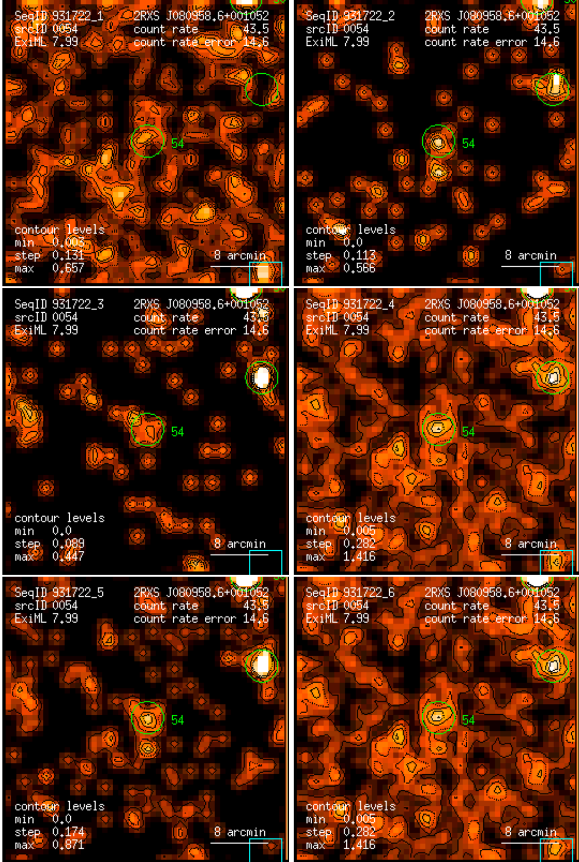
Figure 54: RASS 931722: detection 0054: band rate images, Gaussian filter: (1) PSPC channels 11 – 41, (2) 52 – 90, (3) 91 – 201, (4) 11 – 235, (5) 52 – 201, (6) 11 – 201. Broad band rates in counts/ks. Band rate contour levels in counts/ks/arcmin 2 .
