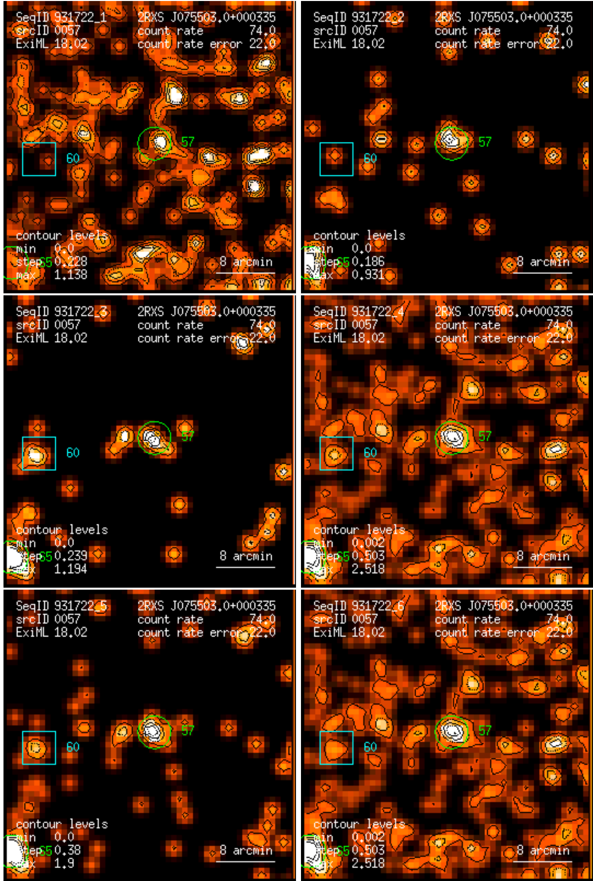
Figure 57: RASS 931722: detection 0057: band rate images, Gaussian filter: (1) PSPC channels 11 – 41, (2) 52 – 90, (3) 91 – 201, (4) 11 – 235, (5) 52 – 201, (6) 11 – 201. Broad band rates in counts/ks. Band rate contour levels in counts/ks/arcmin 2 .
