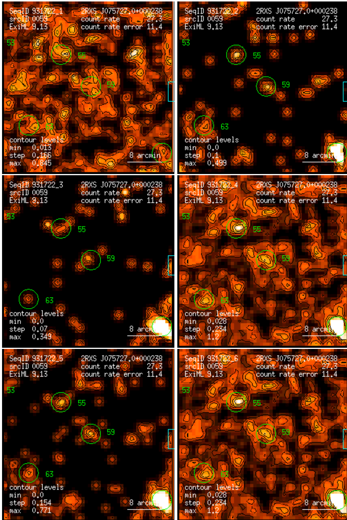
Figure 59: RASS 931722: detection 0059: band rate images, Gaussian filter: (1) PSPC channels 11 – 41, (2) 52 – 90, (3) 91 – 201, (4) 11 – 235, (5) 52 – 201, (6) 11 – 201. Broad band rates in counts/ks. Band rate contour levels in counts/ks/arcmin 2 .
