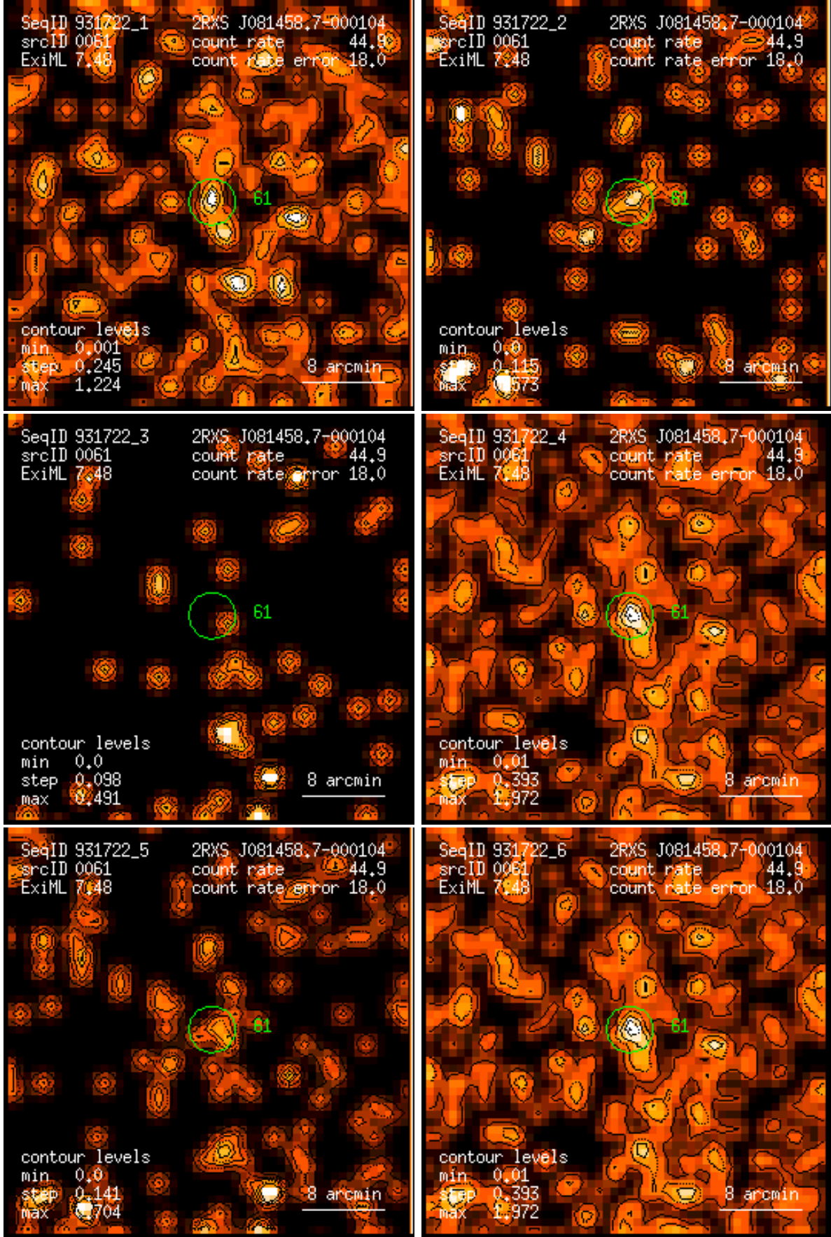
Figure 61: RASS 931722: detection 0061: band rate images, Gaussian filter: (1) PSPC channels 11 – 41, (2) 52 – 90, (3) 91 – 201, (4) 11 – 235, (5) 52 – 201, (6) 11 – 201. Broad band rates in counts/ks. Band rate contour levels in counts/ks/arcmin 2 .
