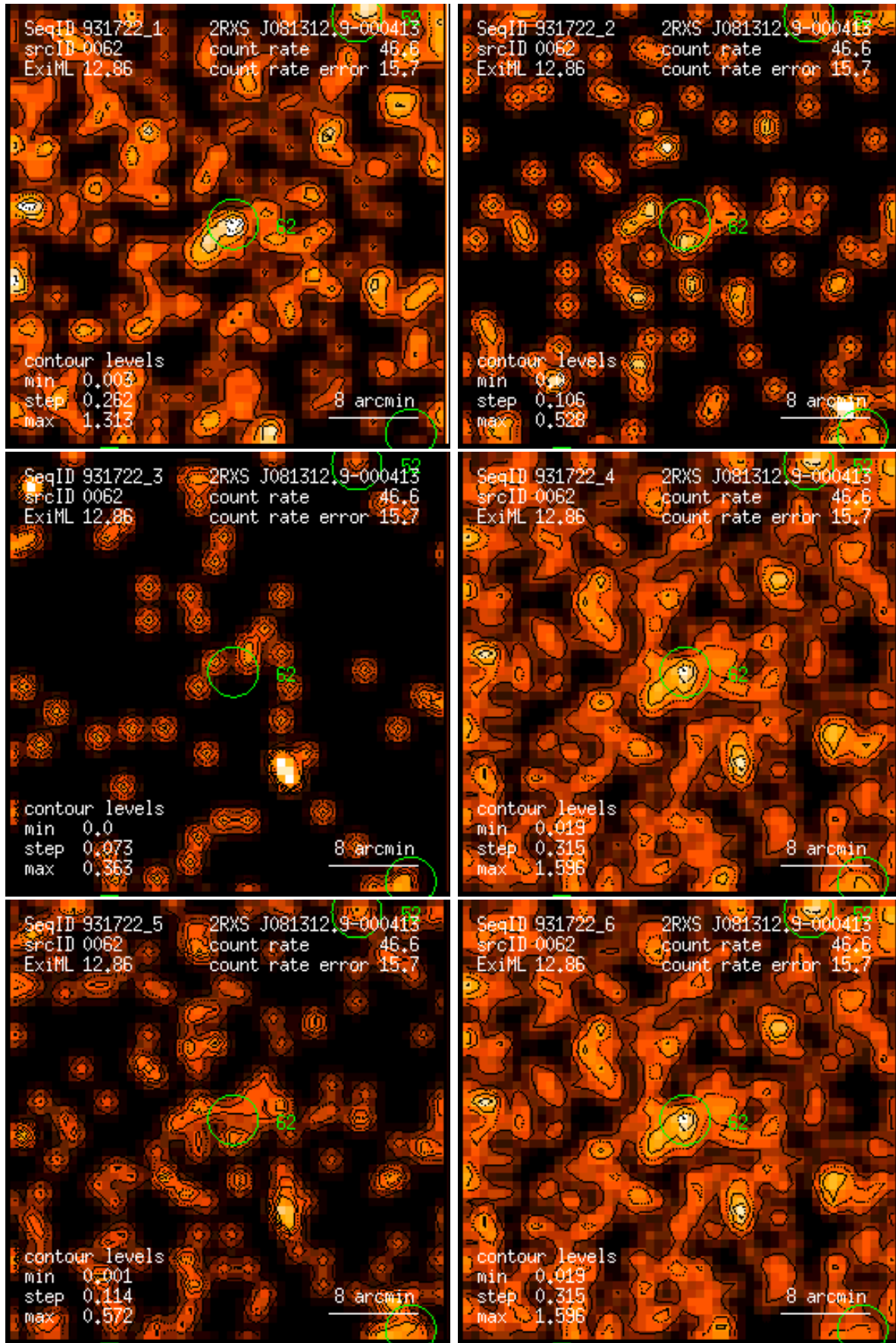
Figure 62: RASS 931722: detection 0062: band rate images, Gaussian filter: (1) PSPC channels 11 – 41, (2) 52 – 90, (3) 91 – 201, (4) 11 – 235, (5) 52 – 201, (6) 11 – 201. Broad band rates in counts/ks. Band rate contour levels in counts/ks/arcmin 2 .
