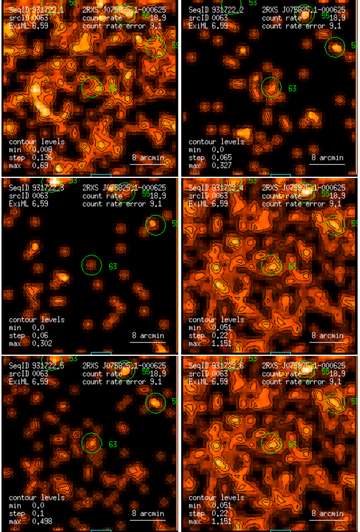
Figure 63: RASS 931722: detection 0063: band rate images, Gaussian filter: (1) PSPC channels 11 – 41, (2) 52 – 90, (3) 91 – 201, (4) 11 – 235, (5) 52 – 201, (6) 11 – 201. Broad band rates in counts/ks. Band rate contour levels in counts/ks/arcmin 2 .
