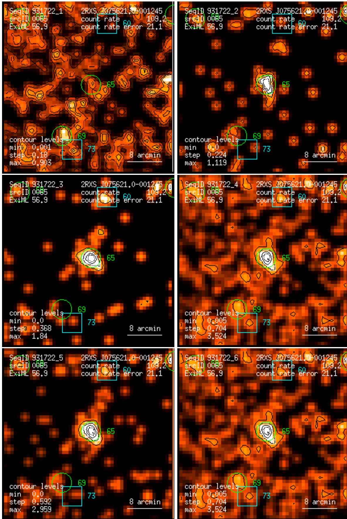
Figure 65: RASS 931722: detection 0065: band rate images, Gaussian filter: (1) PSPC channels 11 – 41, (2) 52 – 90, (3) 91 – 201, (4) 11 – 235, (5) 52 – 201, (6) 11 – 201. Broad band rates in counts/ks. Band rate contour levels in counts/ks/arcmin 2 .
