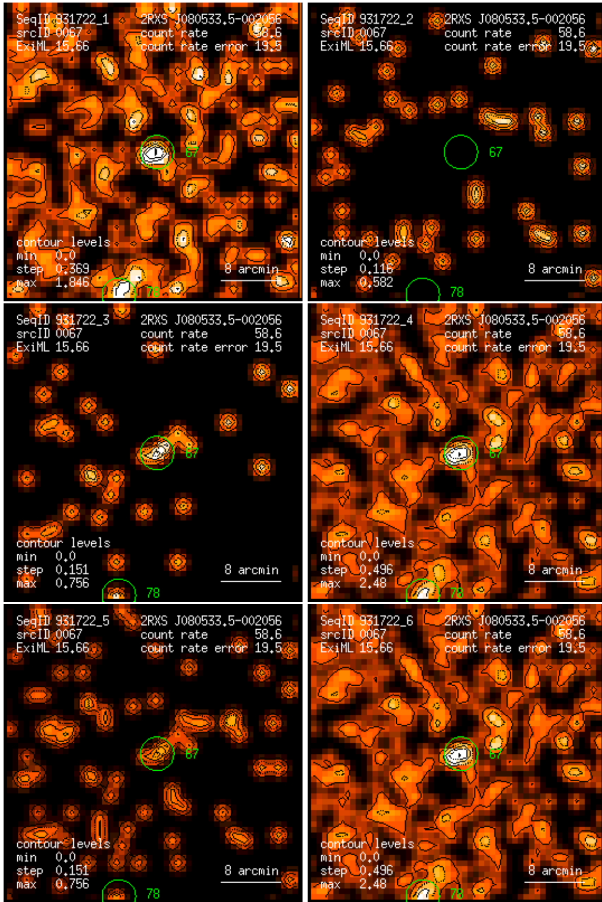
Figure 67: RASS 931722: detection 0067: band rate images, Gaussian filter: (1) PSPC channels 11 – 41, (2) 52 – 90, (3) 91 – 201, (4) 11 – 235, (5) 52 – 201, (6) 11 – 201. Broad band rates in counts/ks. Band rate contour levels in counts/ks/arcmin 2 .
