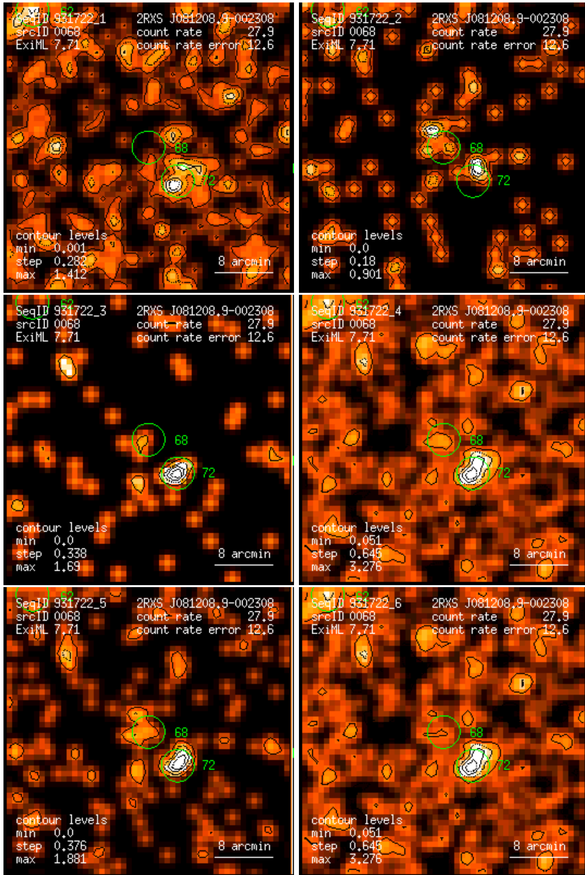
Figure 68: RASS 931722: detection 0068: band rate images, Gaussian filter: (1) PSPC channels 11 – 41, (2) 52 – 90, (3) 91 – 201, (4) 11 – 235, (5) 52 – 201, (6) 11 – 201. Broad band rates in counts/ks. Band rate contour levels in counts/ks/arcmin 2 .
