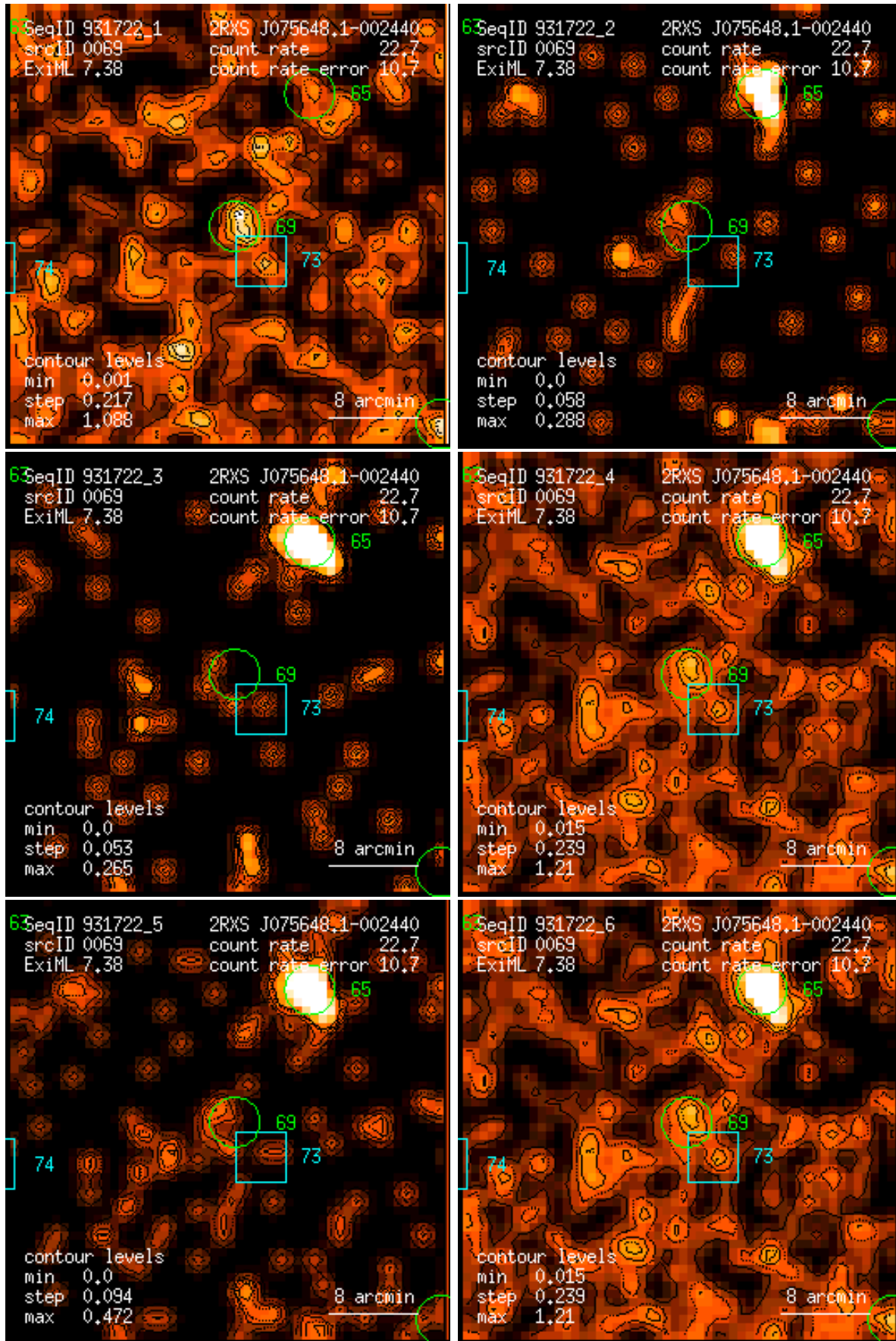
Figure 69: RASS 931722: detection 0069: band rate images, Gaussian filter: (1) PSPC channels 11 – 41, (2) 52 – 90, (3) 91 – 201, (4) 11 – 235, (5) 52 – 201, (6) 11 – 201. Broad band rates in counts/ks. Band rate contour levels in counts/ks/arcmin 2 .
