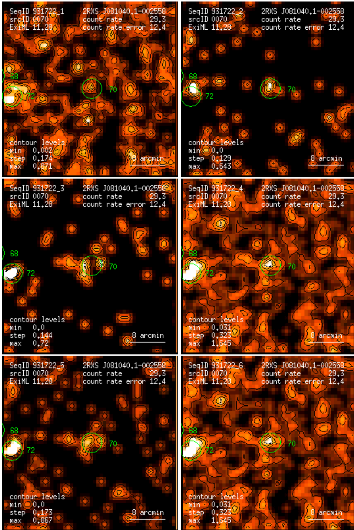
Figure 70: RASS 931722: detection 0070: band rate images, Gaussian filter: (1) PSPC channels 11 – 41, (2) 52 – 90, (3) 91 – 201, (4) 11 – 235, (5) 52 – 201, (6) 11 – 201. Broad band rates in counts/ks. Band rate contour levels in counts/ks/arcmin 2 .
