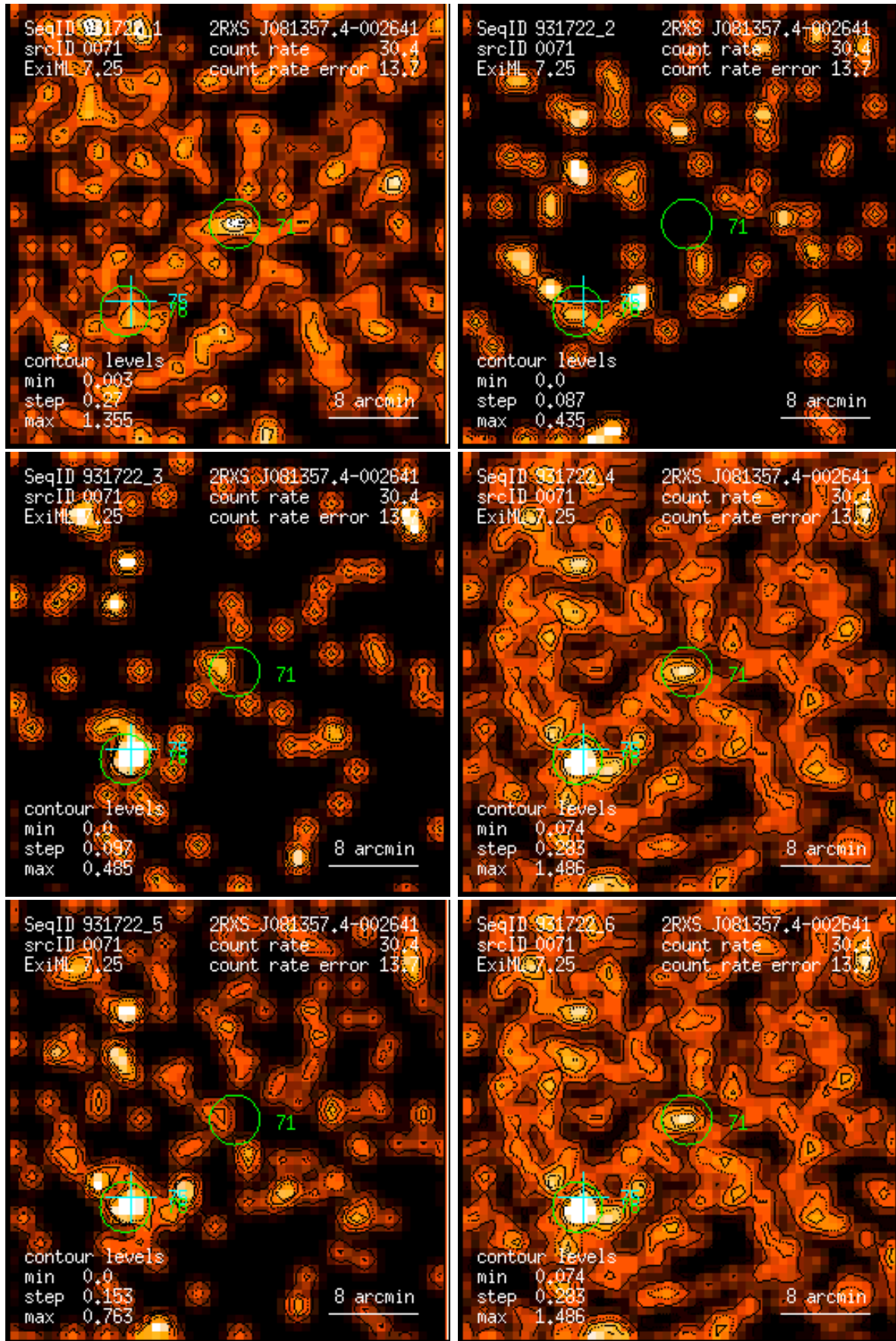
Figure 71: RASS 931722: detection 0071: band rate images, Gaussian filter: (1) PSPC channels 11 – 41, (2) 52 – 90, (3) 91 – 201, (4) 11 – 235, (5) 52 – 201, (6) 11 – 201. Broad band rates in counts/ks. Band rate contour levels in counts/ks/arcmin 2 .
