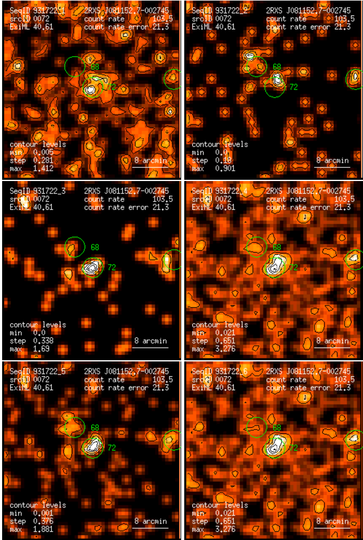
Figure 72: RASS 931722: detection 0072: band rate images, Gaussian filter: (1) PSPC channels 11 – 41, (2) 52 – 90, (3) 91 – 201, (4) 11 – 235, (5) 52 – 201, (6) 11 – 201. Broad band rates in counts/ks. Band rate contour levels in counts/ks/arcmin 2 .
